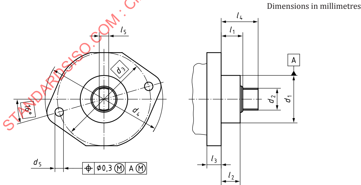
Figure 2 — Type 2 end-mounting flange (with tang drive)
