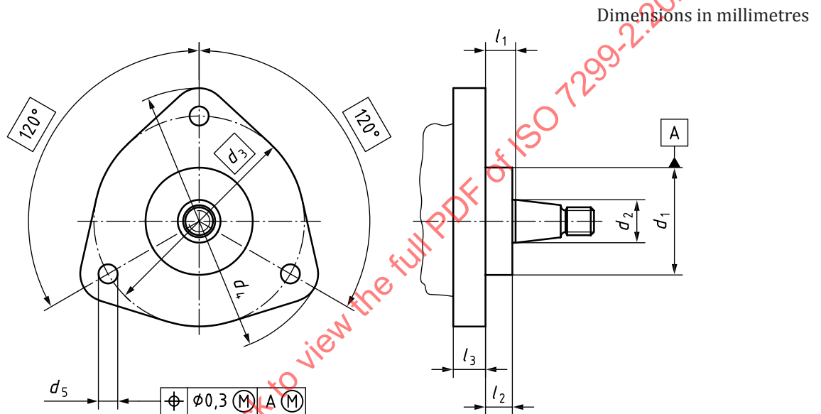
Figure 3 — Type 3 end-mounting flange
