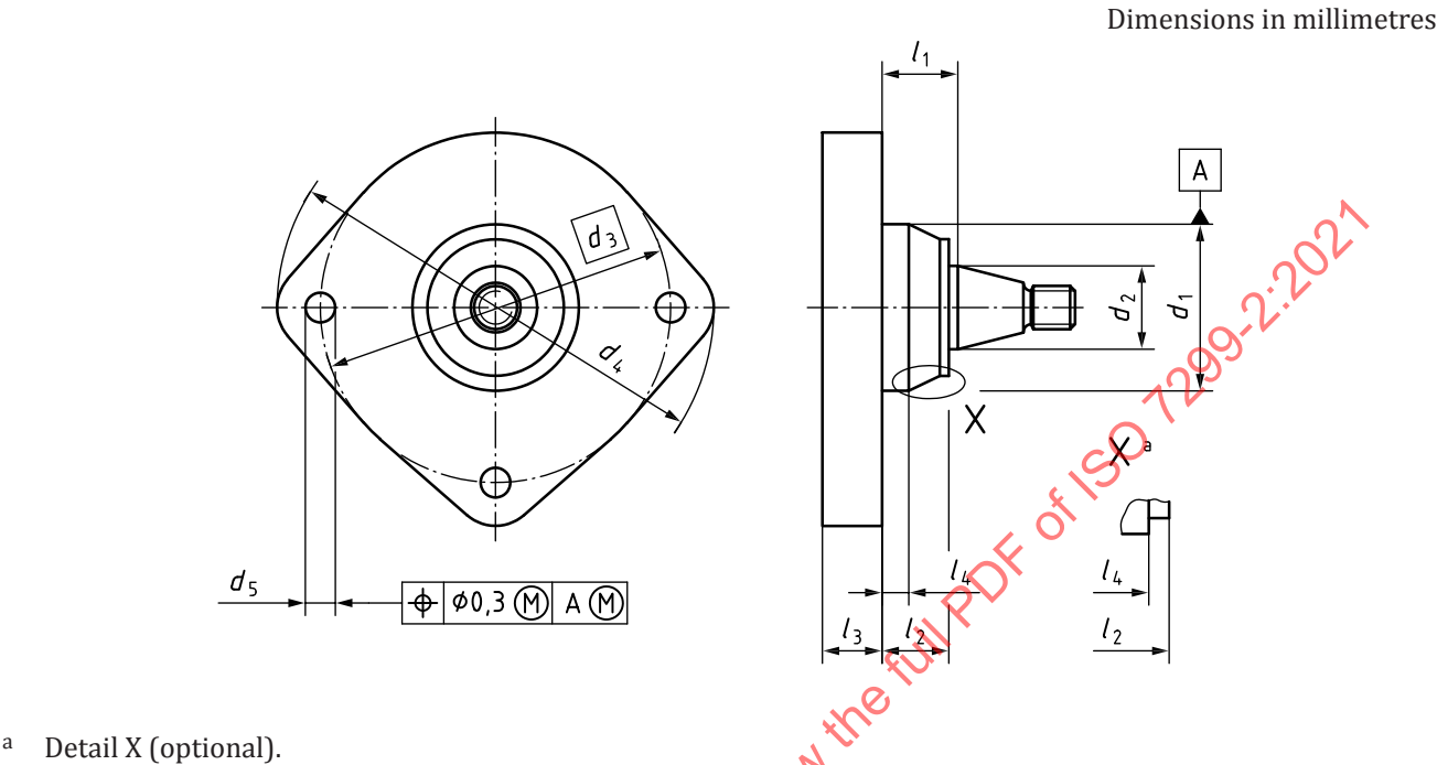
Figure 6 — Type 6 end-mounting flange
