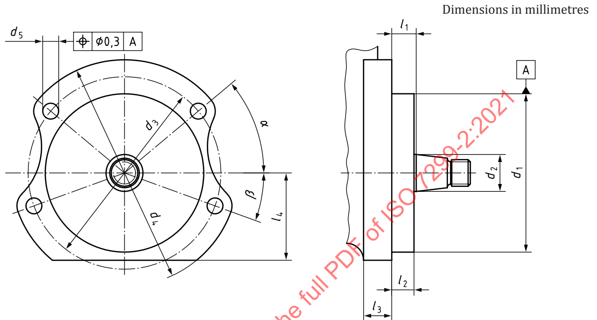
Figure 7 — Type 7 end-mounting flange
