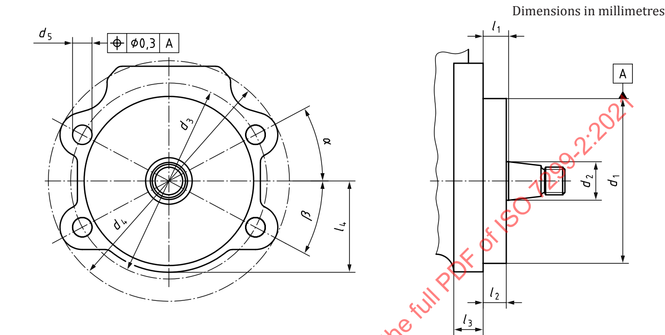
Figure 8 — Type 8 end-mounting flange
