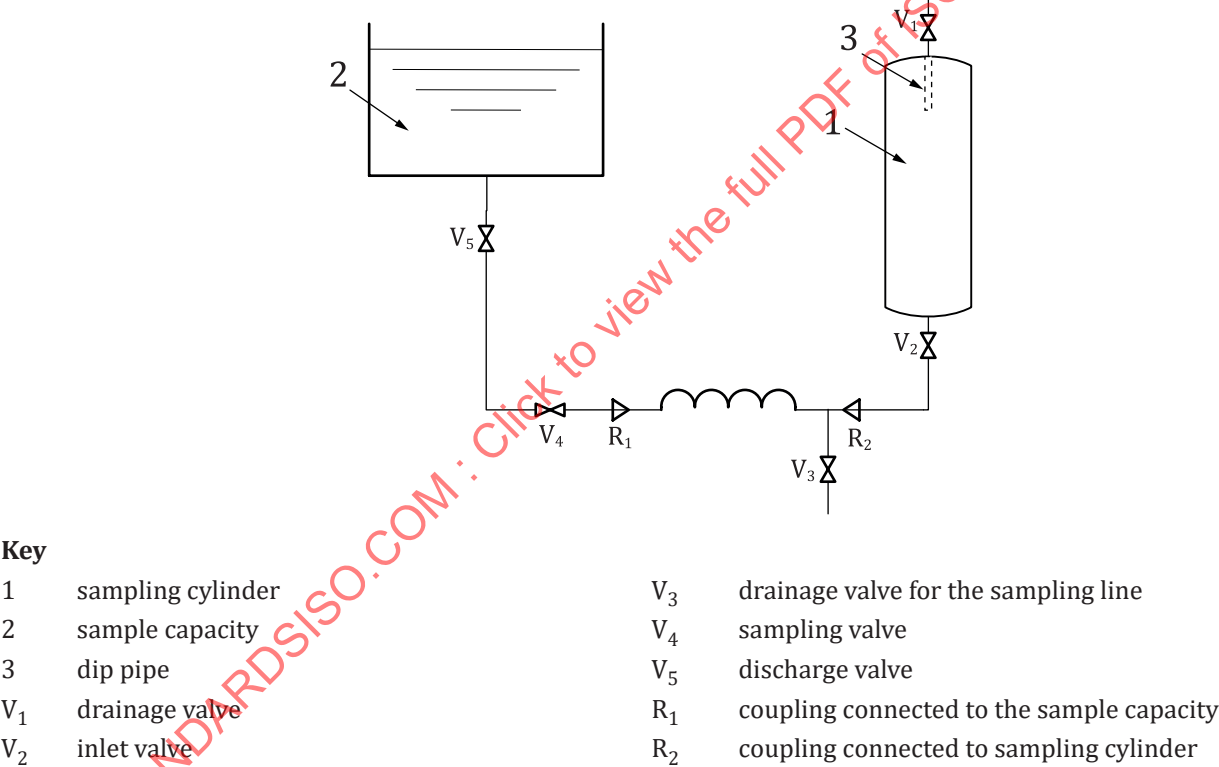
Figure B.1 — Example of non-closed sampling apparatus
