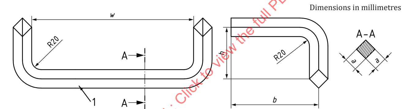
Figure 1 — Example of structure of type A
