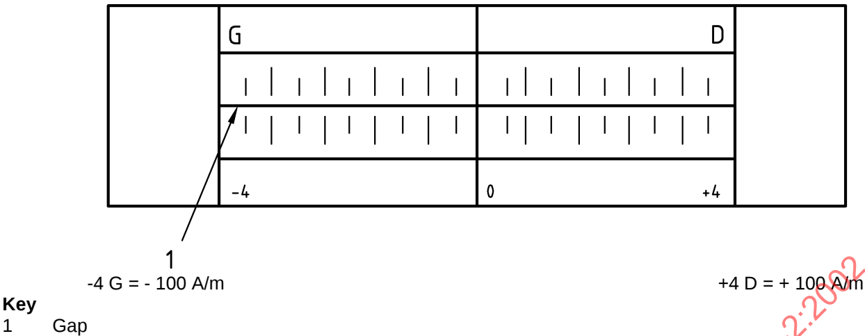
Figure B.4 - Engraving of reference block type 2
