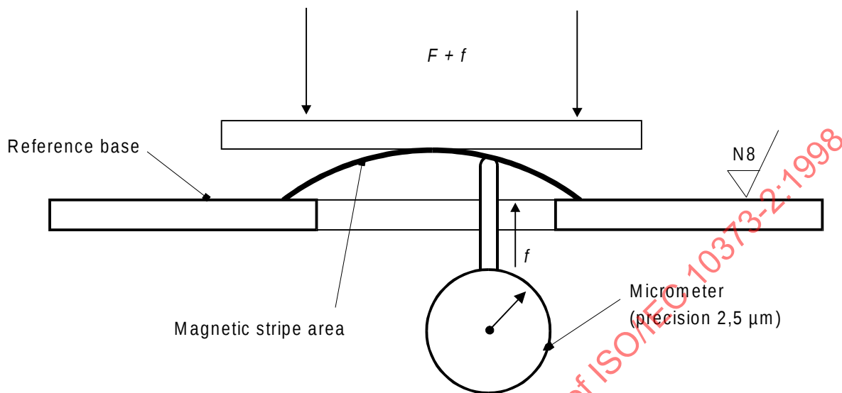
Figure 1 — Measuring arrangement
