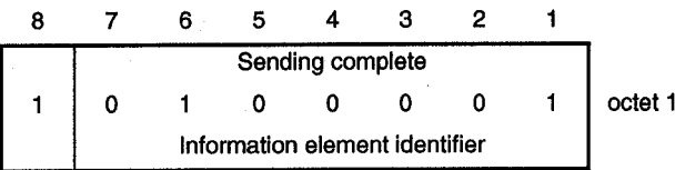
Figure 25 — Sending complete information element
