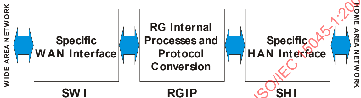
Figure A.2 – Unit architecture
