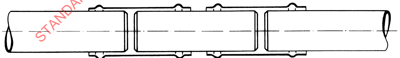
c) Slip-couplers moved into position and make-up piece centralized
