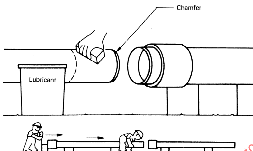
Figure 10 — Example of making a push-fit joint outside the trench
