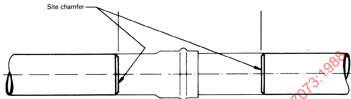
a) Faulty joint cut out and pipe ends chamfered
