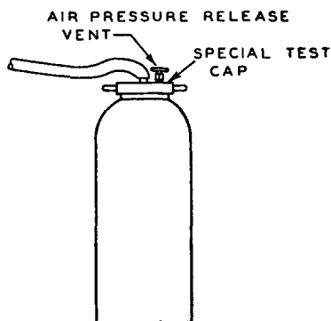
Figure A-5-5.3c. Hydrostatic Testing of Extinguisher Through Fill Collar.
