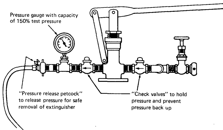
Figure A-5-5.3a. Hydrostatic Hand Pump.
