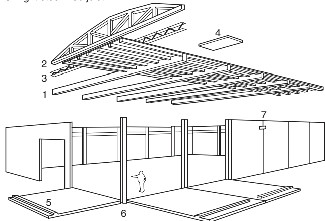
FIGURE D.1(g) Steel Frame with Unreinforced Masonry (URM) In-Fill.
