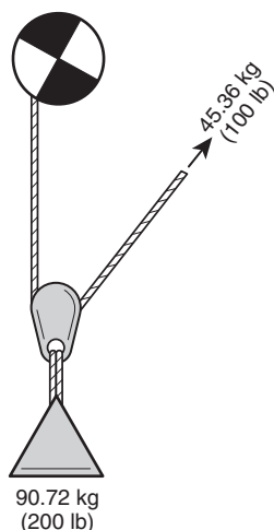
FIGURE A.3.3.119.2 A Simple 2:1 System.
