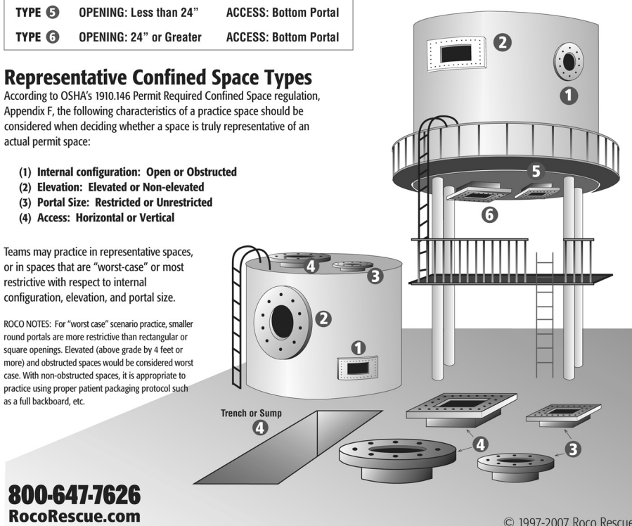
FIGURE A.3.3.38 Confined Space Types.
