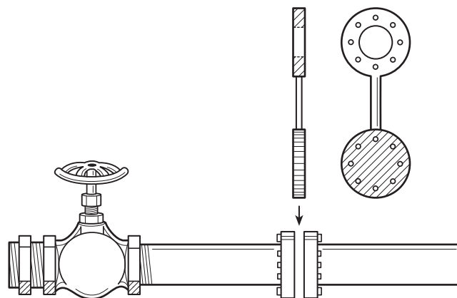
FIGURE A.7.2.2 Blanking or Blinding.
