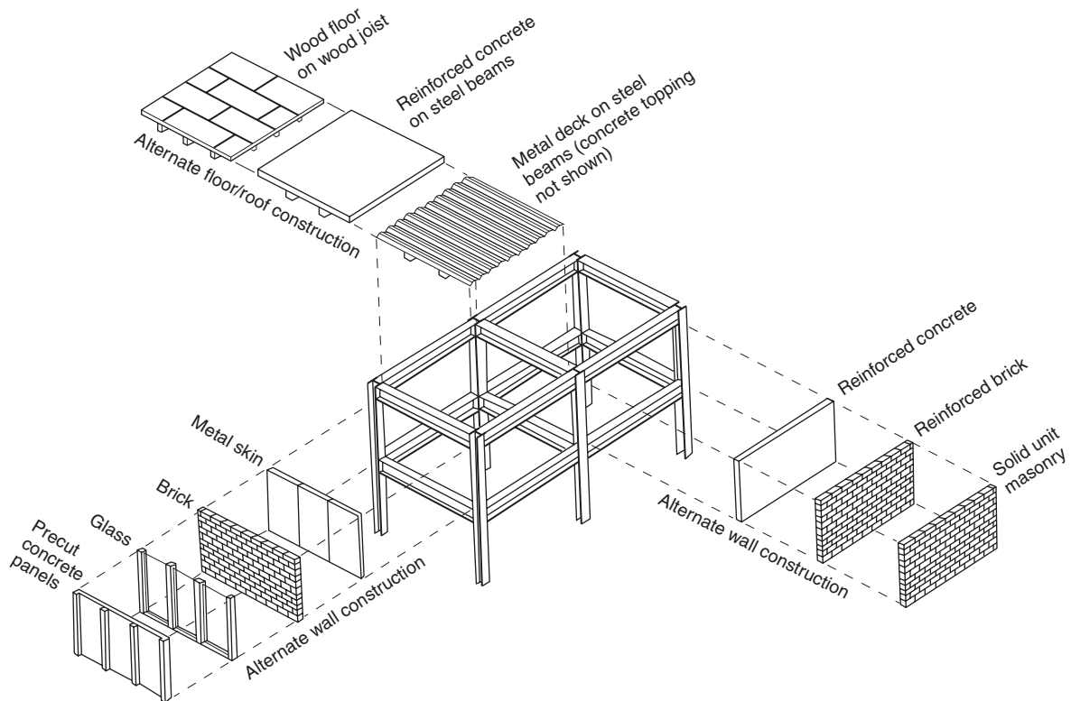
FIGURE D.1(d) Steel Moment-Resisting Frame.
