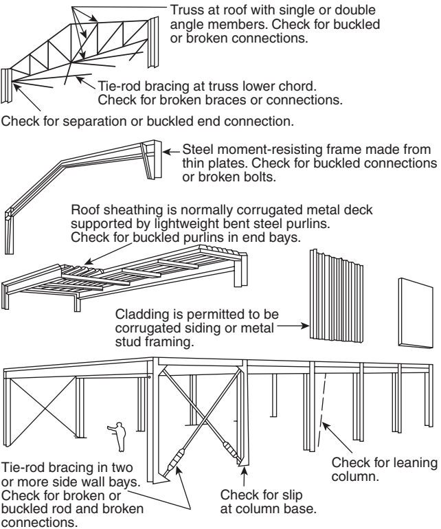
FIGURE D.1(a) Light Metal Buildings.
