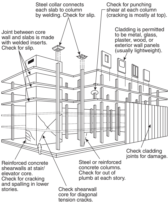
FIGURE D.1(b) Post-Tensioned Lift Slab Building.
