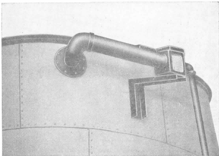
Fig. A-34-31-A. Air Foam Maker in Horizontal Position at Top of Storage Tank.
