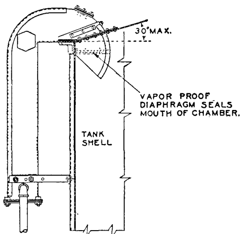
Fig. A-33-13. Roof Entry Outlet.
