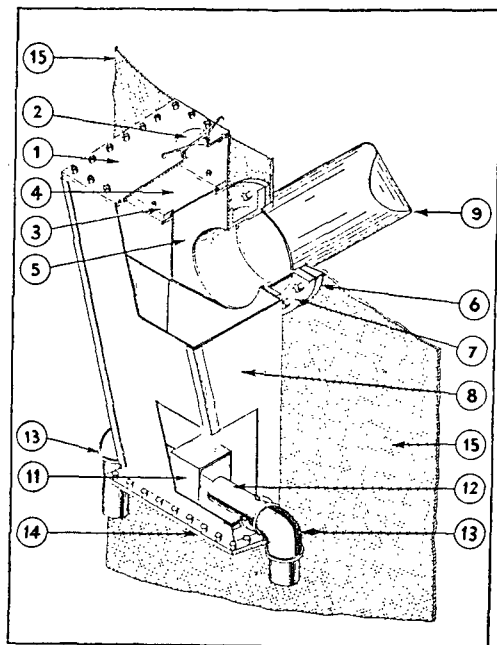
Fig. A-30-23-B. Chemical Foam Chamber. (1) Top plate. (2) Inspection cap. (3) Diaphragm Frame. (4) Diaphragm. (5) Inner Chamber. (6) Adapter flange shaped to fit tank curvature. (7) Chamber throat and mounting flange. (8) Chamber body. (9) Deflector. (11) Baffle. (12) Inlet nipples. (13) Inlet solution elbows. (14) Bottom plate. (15) Tank Shell.
