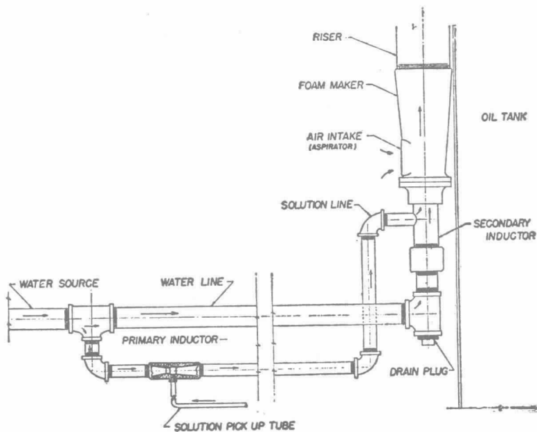
Fig. A-11-55.33. Air Foam Auto-Induction System. Solution pick-up tube picks up stabilizer from its container.
