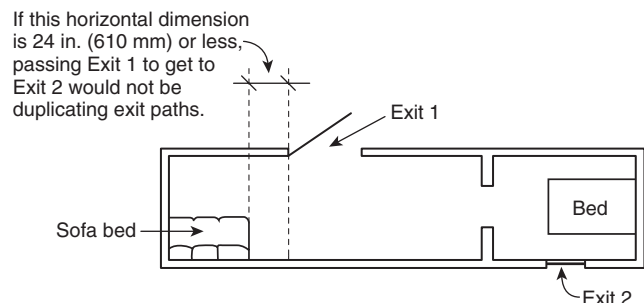
FIGURE A.6.2.1 Bed Within 24 in. (610 mm) of the Plane of the Nearest Designated Exit.
