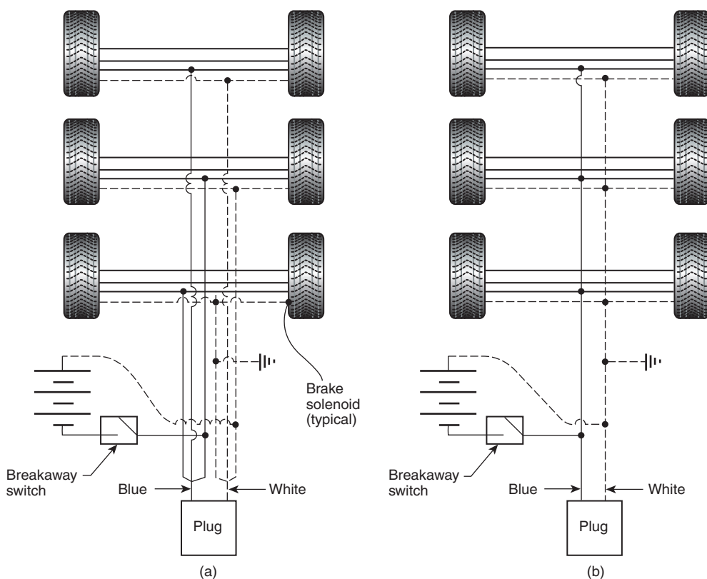
▲ FIGURE 8.4.1.7 Brake Wiring Diagram. [© CSA Z240]
