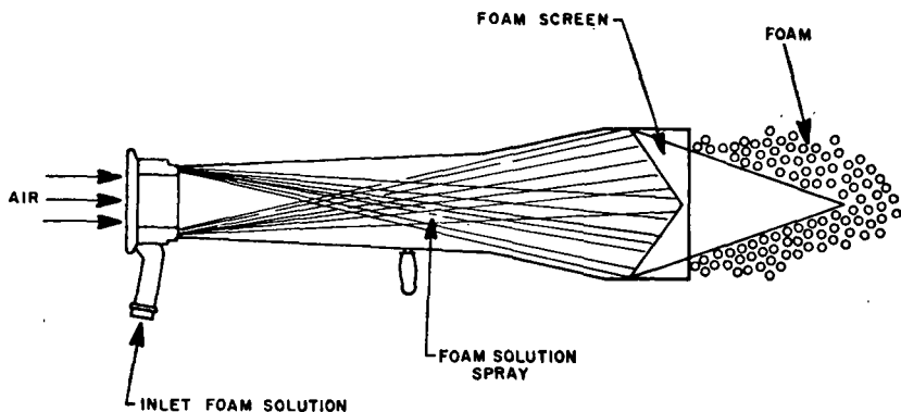
Figure A-1-9.5(b) Aspirating Type Foam Generator
