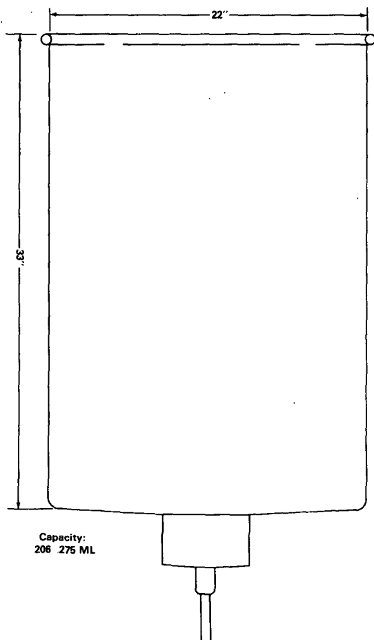
Figure A-1-10.5(b)(2) Drainage Drum for High Expansion Foam Expansion and Drainage Test.
