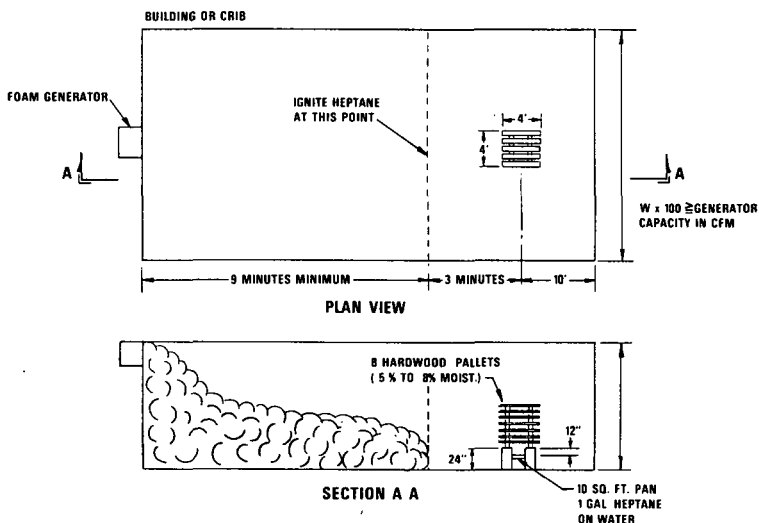
Figure A-1-10.5(a) Fire Performance Test
