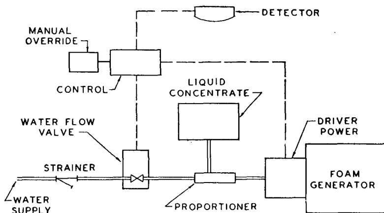
Figure A-1-9.5(a) Block Diagram of Automatic High Expansion Foam System
