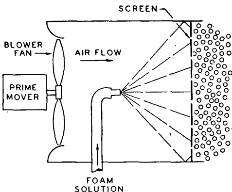
Figure A-1-9.5(c) Blower Type Foam Generator
