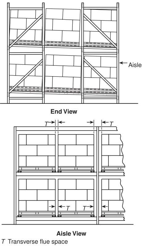
FIGURE A.3.3.177(g) Flow-Through Pallet Rack.
