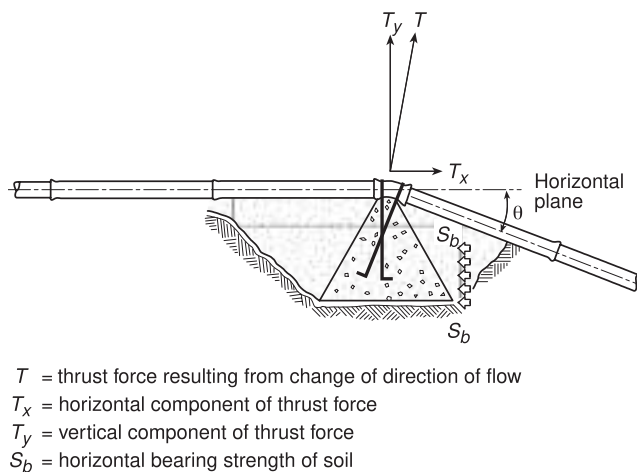
FIGURE A.6.6.1(c) Gravity Thrust Block. [24:Figure A.10.6.1(c)]
