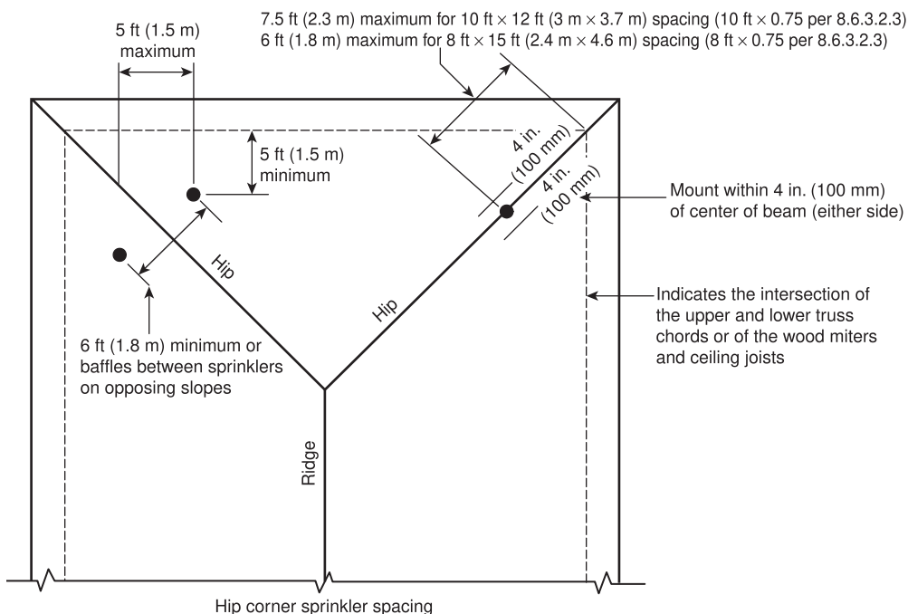
FIGURE A.10.2.6.1.4.5 Hip Roof Installations.
