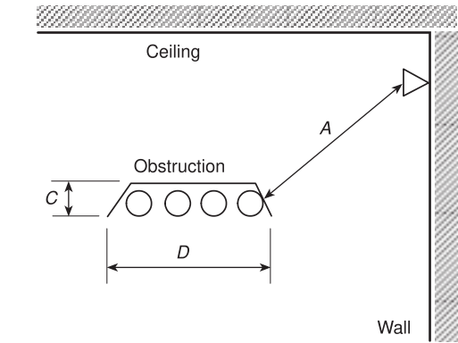
Elevation View of Pipe Conduit or Light Fixture (Obstruction in horizontal orientation) A \geq 4C \text{ or } 4D A \leq 36 \text{ in. (900 mm)} (Use dimension C or D , whichever is greater)
