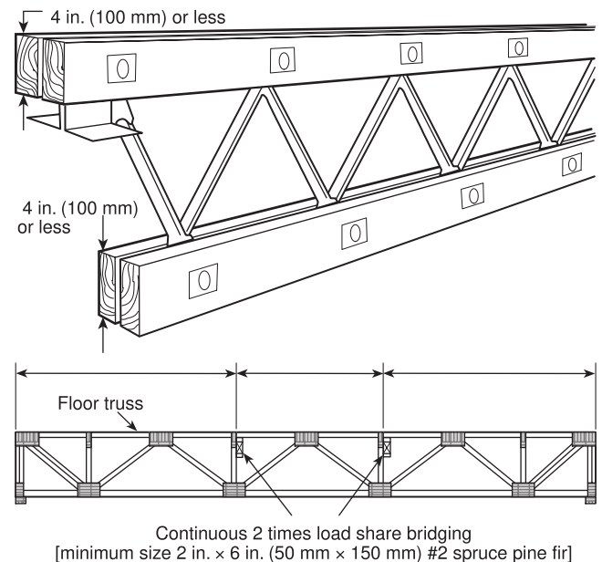
▲ FIGURE A.3.3.43.2(c) Examples of Wood Truss Construction.
