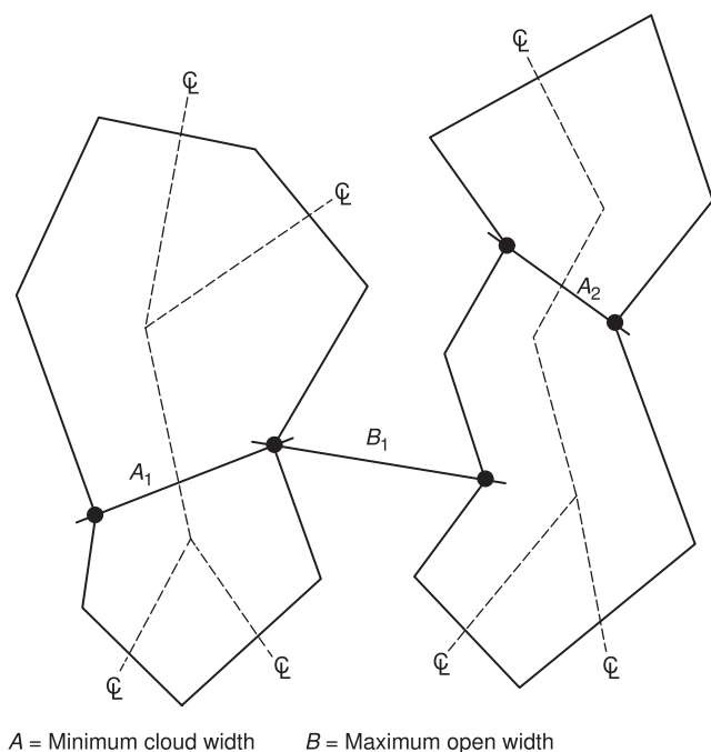
Δ FIGURE A.9.2.7.2.5 Irregular Shaped Cloud Dimensioning.
