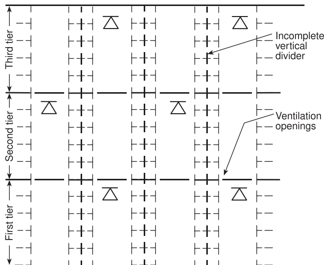
FIGURE 9.3.7(b) Sprinklers in Multitier Bookshelves with Incomplete Vertical Dividers.
