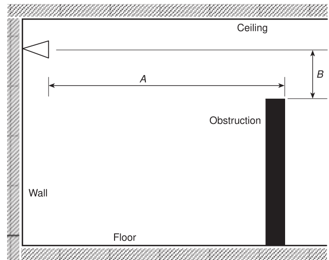
Elevation View
