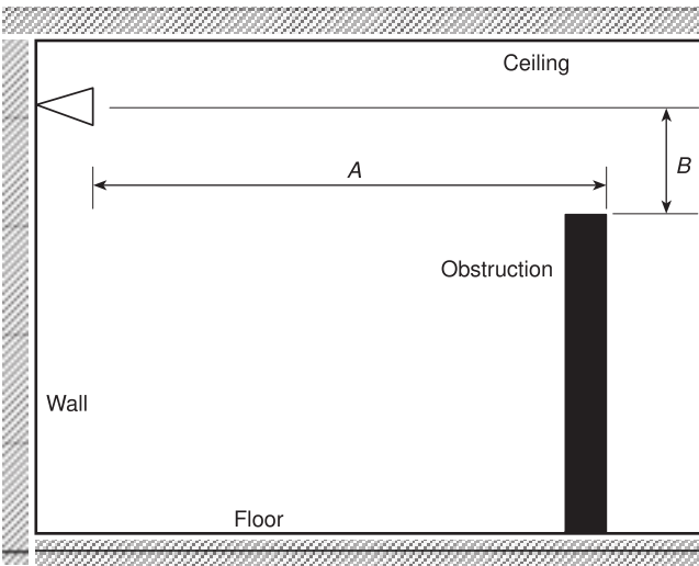
Elevation View
