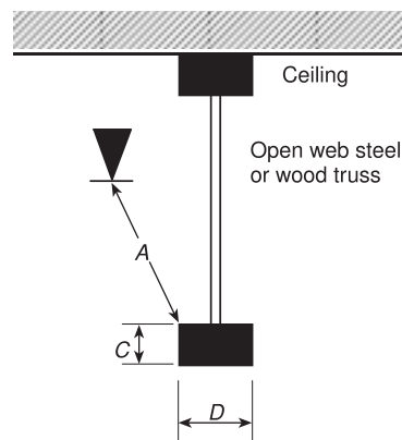
FIGURE 10.2.7.3.1.3(b) Minimum Distance from an Obstruction in the Horizontal Orientation (SSU/SSP).
