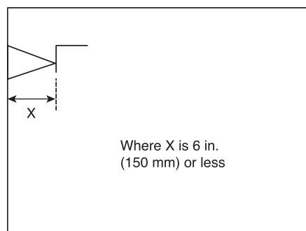
FIGURE A.10.3.5.1.2.1 Sidewall Sprinkler Deflector Measurement From Walls.
