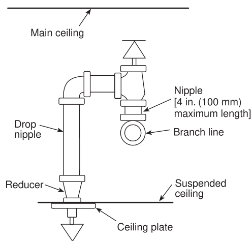
FIGURE 30.4.5 Sprinklers in Concealed Space and Below Ceiling.
