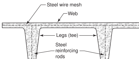
FIGURE A.3.3.43.1(a) Typical Concrete Tee Construction.
