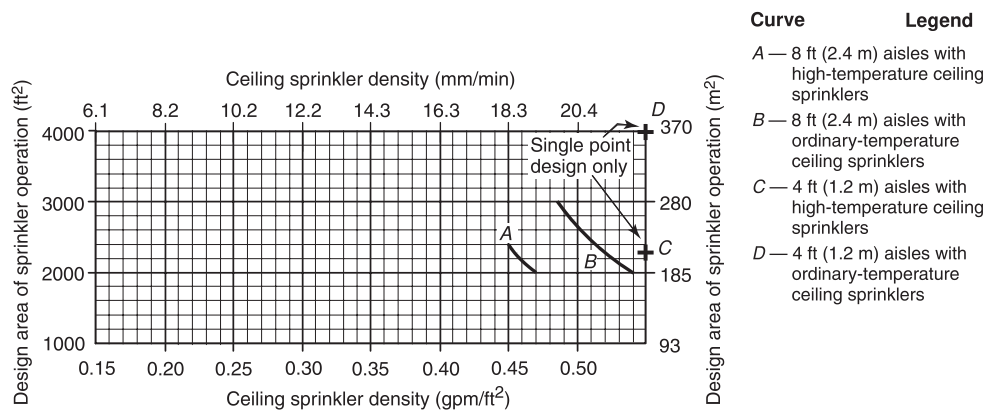
FIGURE 21.4.1.2.1(e) Single- or Double-Row Racks — 20 ft (6.1 m) High Rack Storage — Sprinkler System Design Curves — Class I and Class II Encapsulated Commodities — Conventional Pallets.
