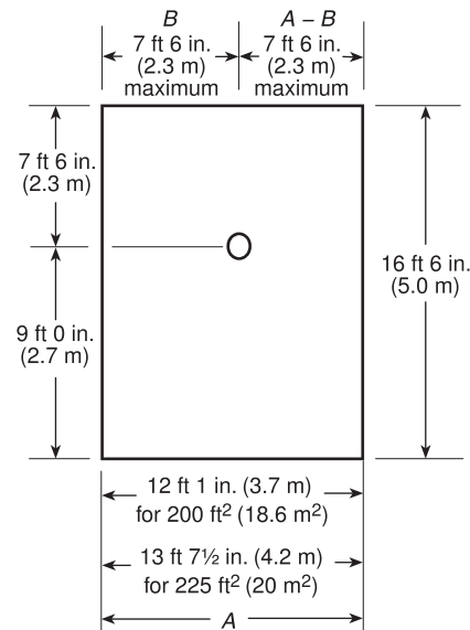
FIGURE A.10.2.5.2.3(a) Small Room Provision — One Sprinkler.
