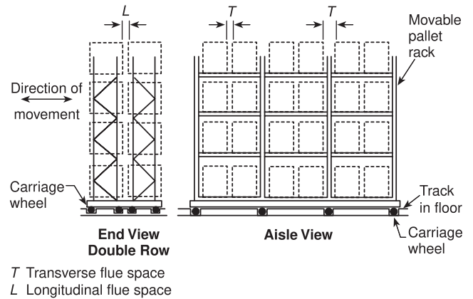
FIGURE A.3.3.177(k) Movable Rack.
