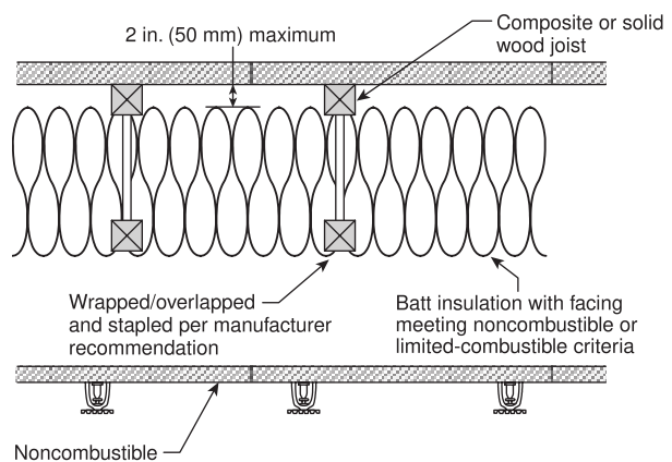
FIGURE A.9.2.1.19 Acceptable Arrangement of Concealed Space Not Requiring Sprinklers.
