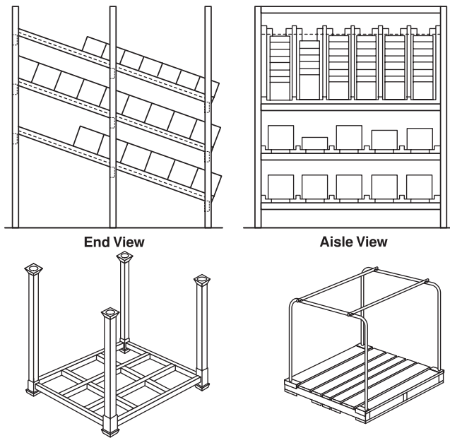
FIGURE A.3.3.177(i) Flow-Through Racks (Top) and Portable Racks (Bottom).
