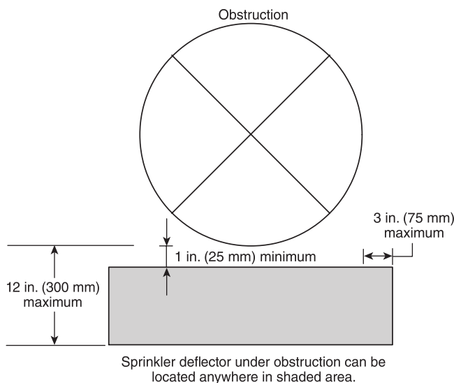
FIGURE A.9.5.5.3.1.2(b) Sprinkler Location Below Circular Obstruction.
