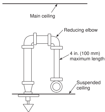
FIGURE 30.4.4 Nipple and Reducing Elbow Supplying Sprinkler Below Ceiling.
