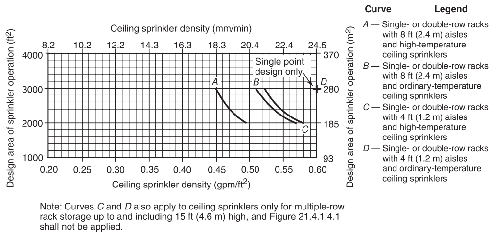
FIGURE 21.4.1.2.1(d) Sprinkler System Design Curves — 20 ft (6.1 m) High Rack Storage — Class IV Nonencapsulated Commodities — Conventional Pallets.
