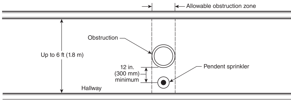
N FIGURE 10.2.7.2(d) Obstruction in Hallway.
