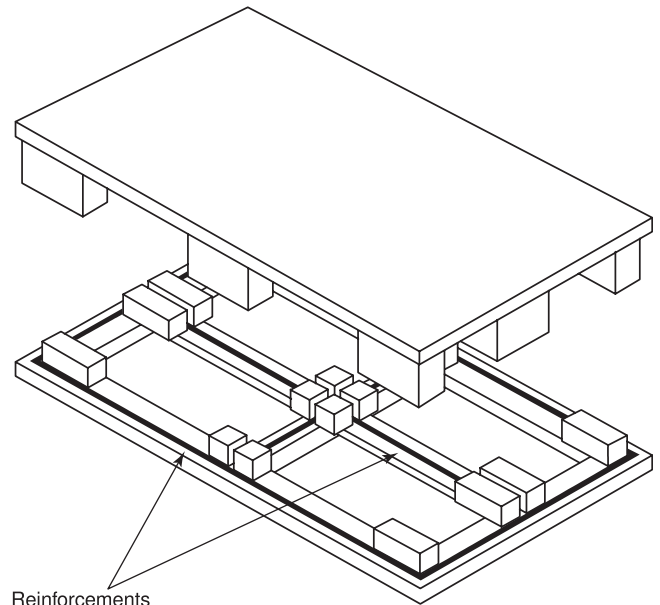
FIGURE A.3.3.154.3(a) Cut-Away Reinforced Plastic Pallet.
