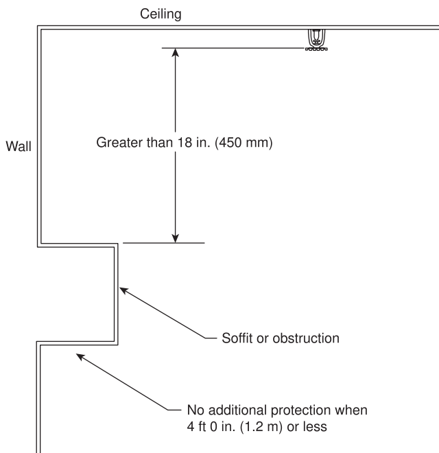
FIGURE A.10.2.7.2 Soffit/Obstruction Against Wall Greater Than 18 in. (450 mm) Below Deflector.
