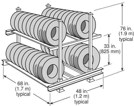
Δ FIGURE A.3.3.191(c) Open Portable Tire Rack.
