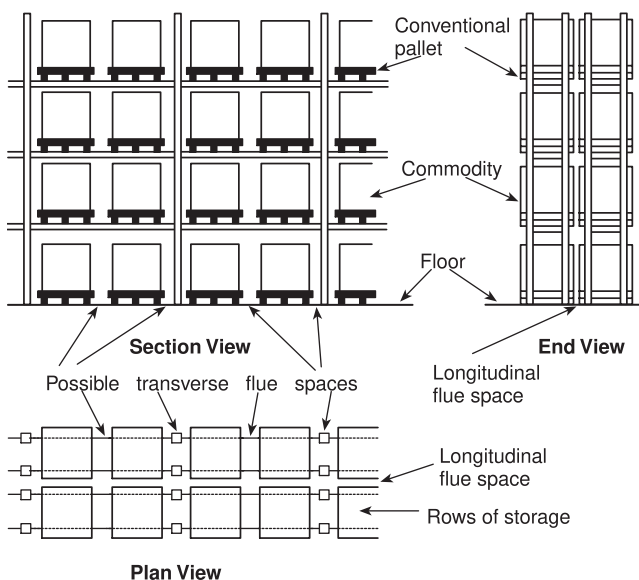
FIGURE A.3.3.122 Typical Double-Row (Back-to-Back) Rack Arrangement.
