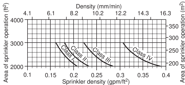
FIGURE 21.2.2.3.1 For the Evaluation or Modification of Existing Systems, Sprinkler System Design Curves for 20 ft (6.1 m) High Storage — Ordinary Temperature-Rated Sprinklers.
