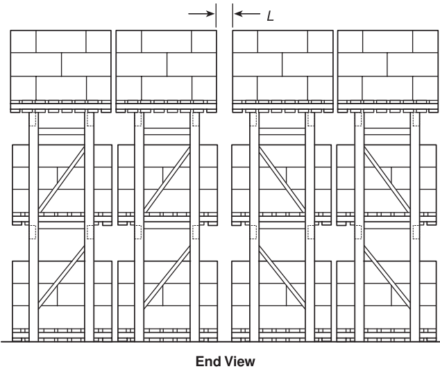
FIGURE A.3.3.177(f) Multiple-Row Rack Served by Reach Truck.
