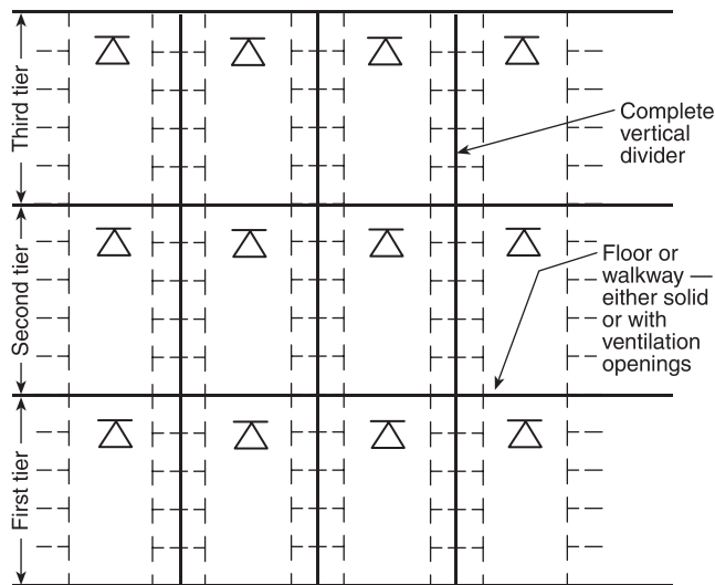
FIGURE 9.3.7(a) Sprinklers in Multitier Bookshelves with Complete Vertical Dividers.
