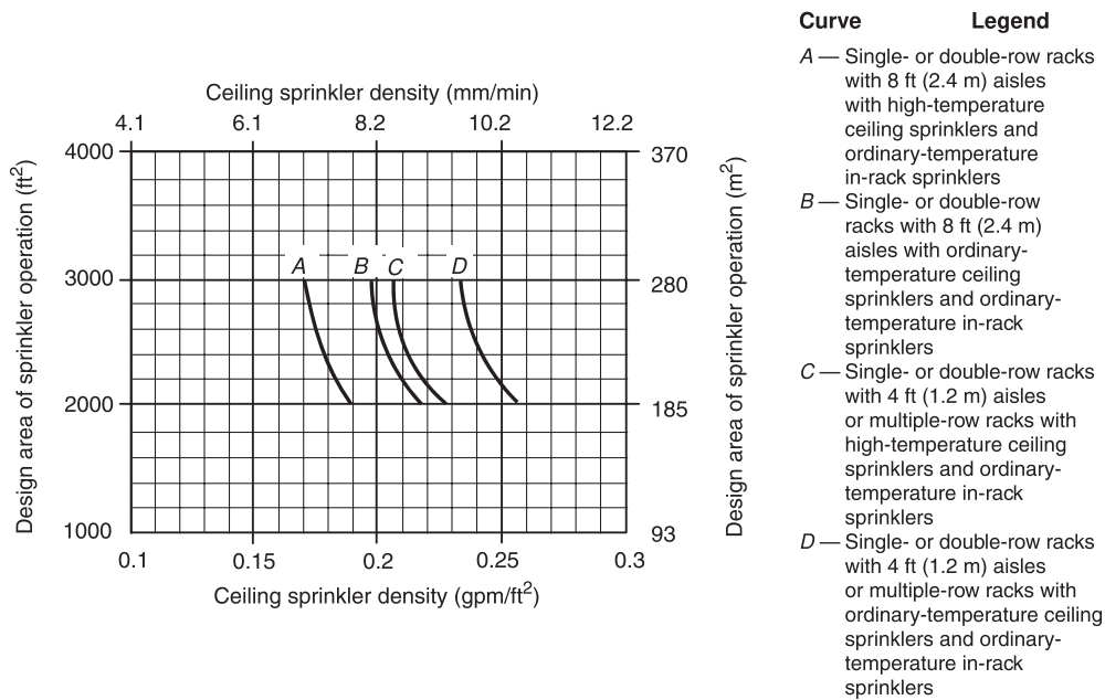
N FIGURE 25.8.2.2.1(a) CMDA Sprinkler System Design Curves — 20 ft (6.1 m) High Rack Storage — Exposed Nonencapsulated Class I Commodities — Conventional Pallets.
