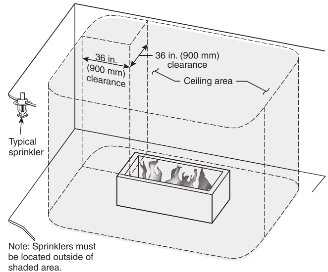
FIGURE A.9.4.2.5(c) Ordinary-Temperature Sprinkler over Open Fireplace.
