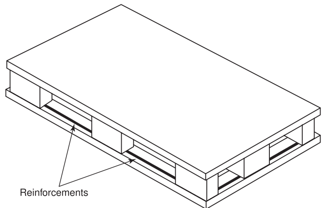
FIGURE A.3.3.154.3(b) Assembled Reinforced Plastic Pallet.
