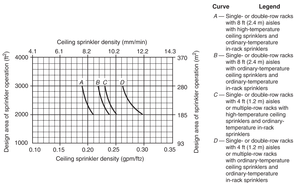
N FIGURE 25.8.2.2.1(b) CMDA Sprinkler System Design Curves — 20 ft (6.1 m) High Rack Storage — Exposed Nonencapsulated Class II Commodities — Conventional Pallets.
