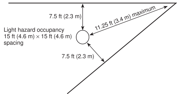
FIGURE A.10.2.5.2.2 Maximum Distance from Walls.
