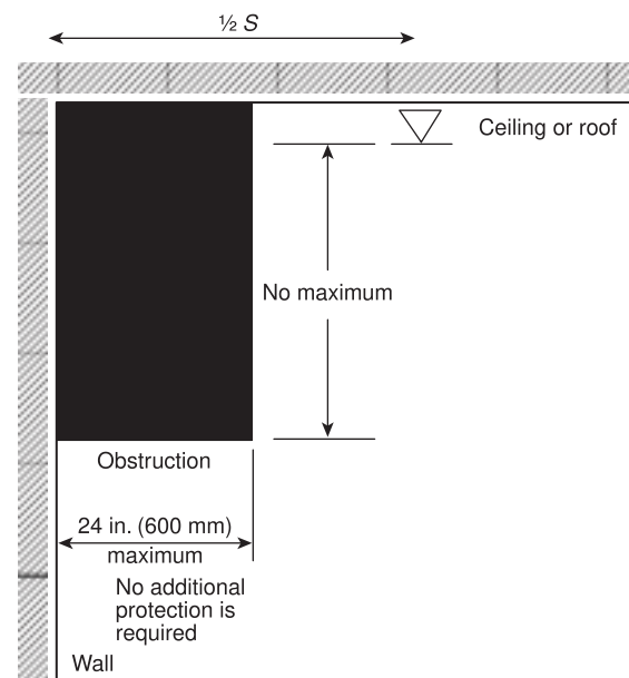
FIGURE 10.2.7.2(c) Obstructions Against Walls (SSU/SSP).
