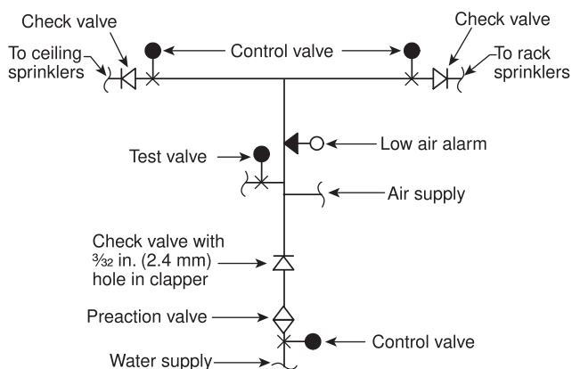
FIGURE 8.8.2.8.4 Valve Arrangement.
