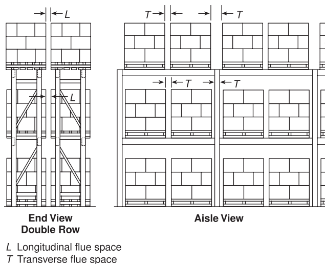
FIGURE A.3.3.177(a) Conventional Pallet Rack.
