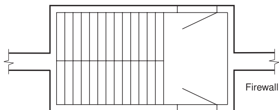
FIGURE A.9.3.4.3(a) Noncombustible Stair Shaft Serving Two Sides of Fire Wall.
