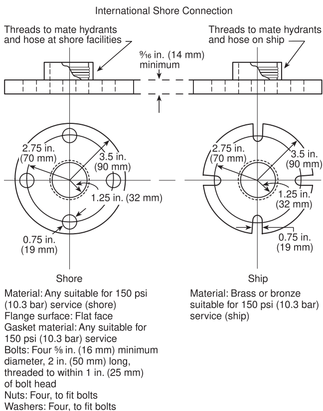
FIGURE A.3.3.125.7 International Shore Fire Connection.
