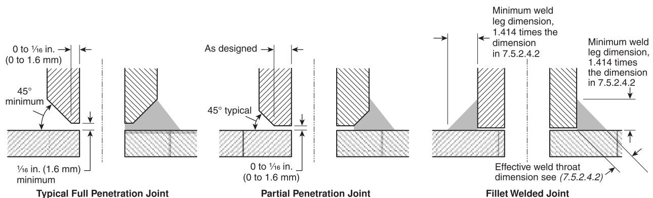
FIGURE A.7.5.2.4.1 Weld Descriptions.
