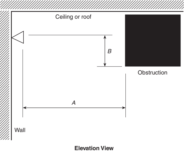
FIGURE 6.4.6.3.5.2(a) Positioning of Sprinklers to Avoid Obstructions (Residential Sidewall Sprinklers).
