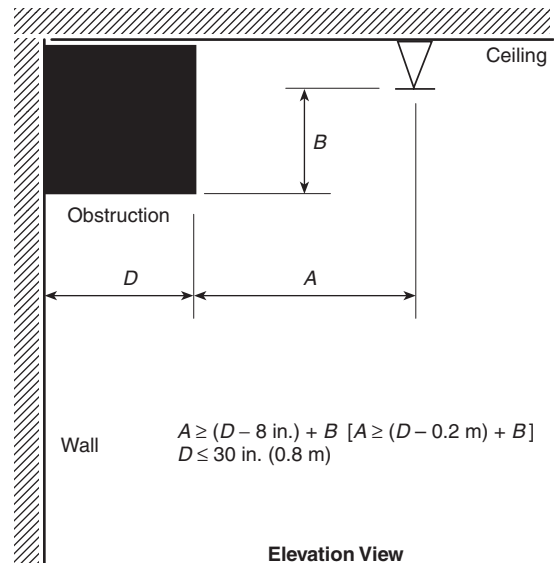
FIGURE 6.4.6.3.4.3 Obstructions Against Walls (Residential Upright and Pendent Spray Sprinklers).
