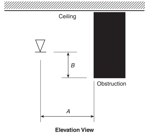
FIGURE 6.4.6.3.4.2 Positioning of Sprinklers to Avoid Obstructions to Discharge (Residential Upright and Pendent Spray Sprinklers).
