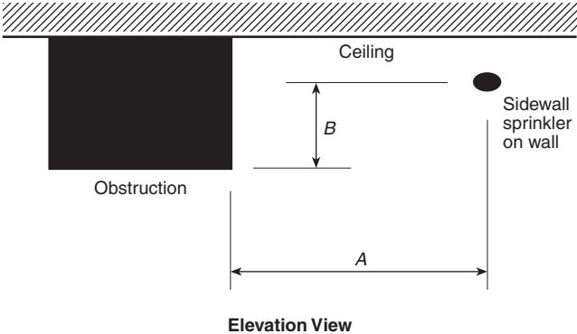
FIGURE 6.4.6.3.5.2(b) Positioning of Sprinklers to Avoid Obstructions Along the Wall (Residential Sidewall Sprinklers).
