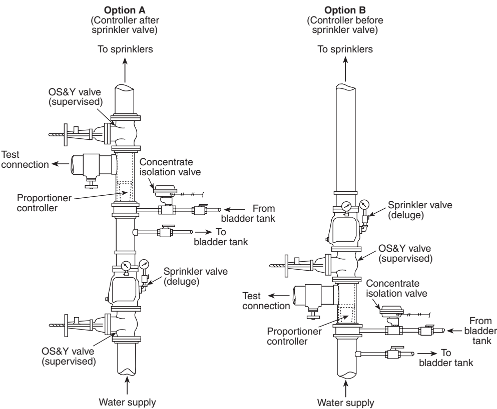
FIGURE A.5.13 Test Connection Detail.
