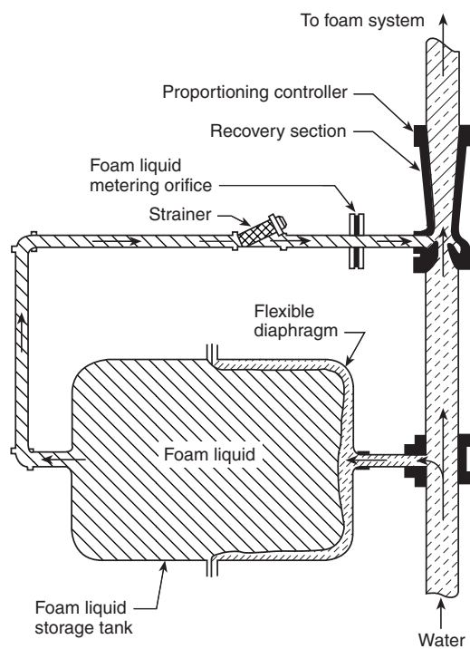
FIGURE A.5.4.2(c) Pressure Proportioning Tank with Diaphragm.
