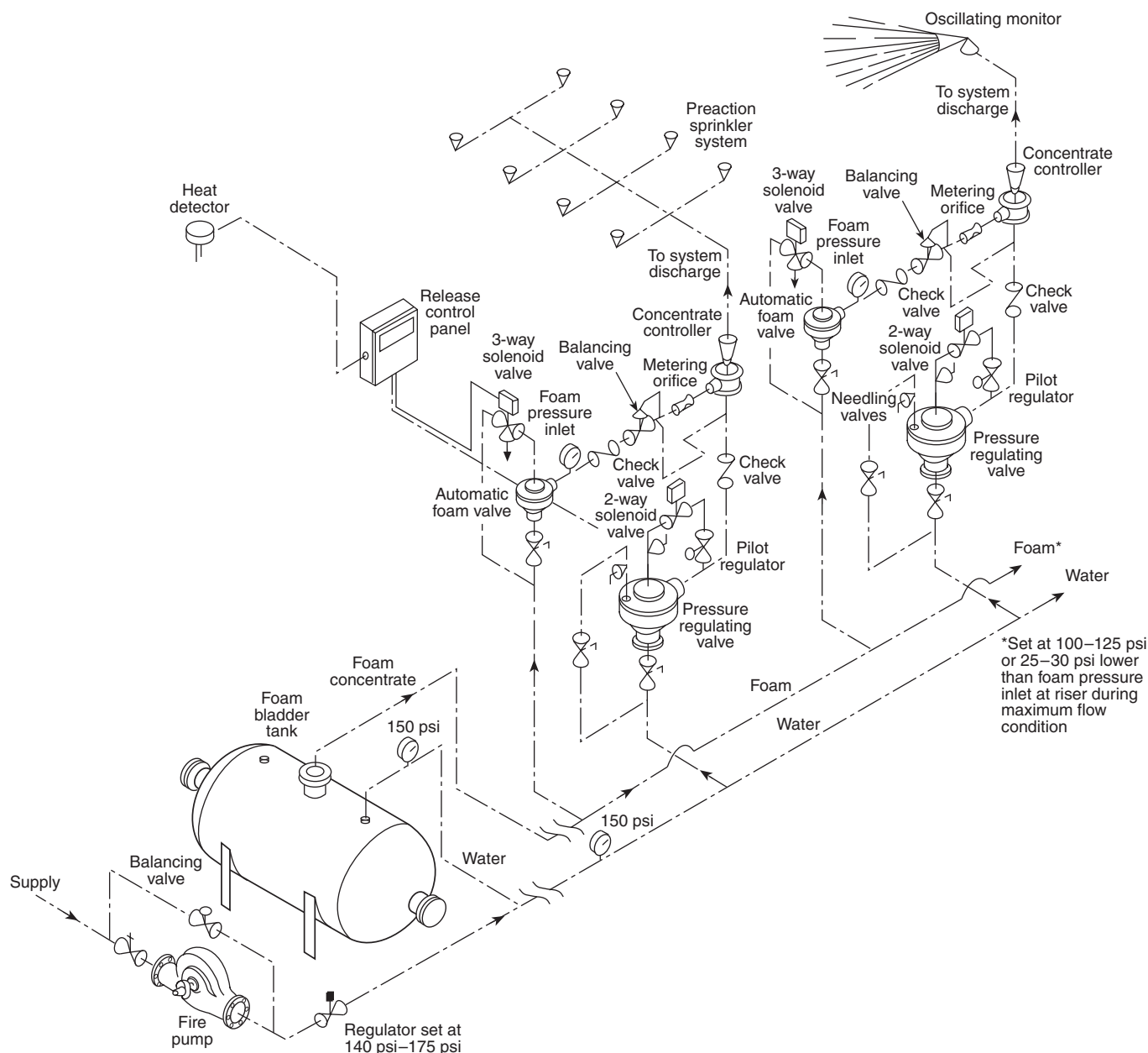
FIGURE A.5.4.2(h) In-Line Balanced-Pressure Proportioning System with Bladder Tank.
