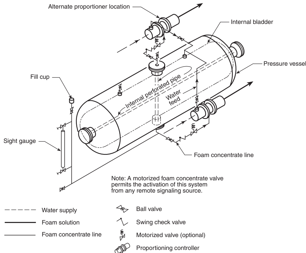
FIGURE A.5.4.2(f) Balanced-Pressure Proportioning (Bladder System).
