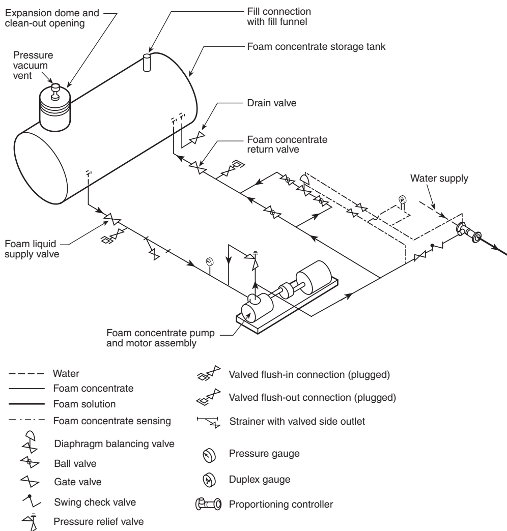
FIGURE A.5.4.2(e) Balanced-Pressure Proportioners (with Concentrate Pump).
