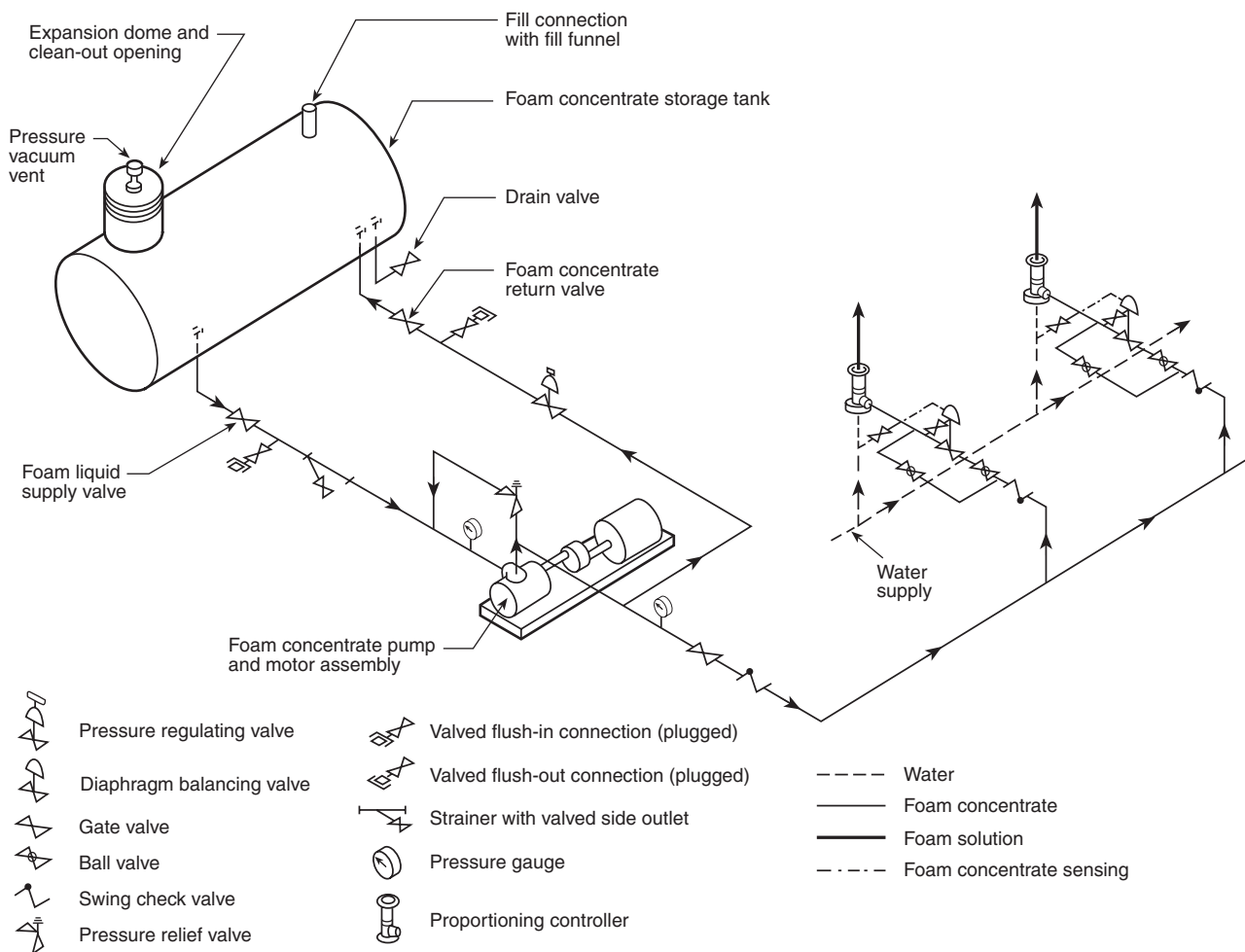
FIGURE A.5.4.2(g) In-Line Balanced-Pressure Proportioning System.
