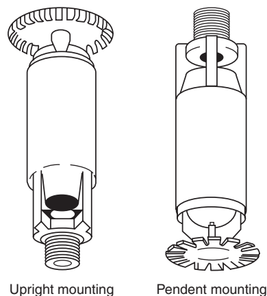
FIGURE A.3.3.7.1 Variations in Deflector Shape.
