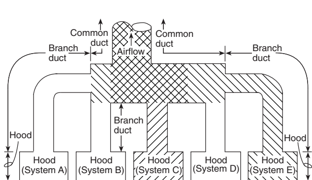
FIGURE A.5.6.2.1(2)(b) Simultaneous Operation of Two Systems in Which One Also Provides Common Duct Protection.
