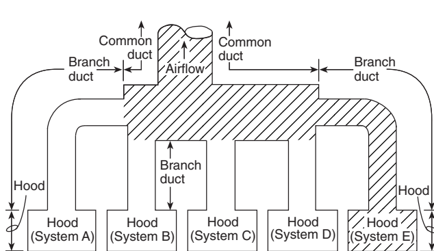
FIGURE A.5.6.2.1(2)(c) Independent Operation of a System That Protects a Hood and the Common Duct.
