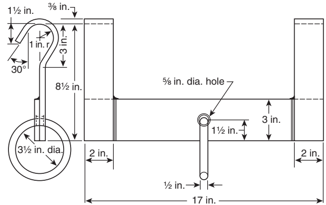
FIGURE A.19.8.7.4.2 Hanger for Test Cable.
