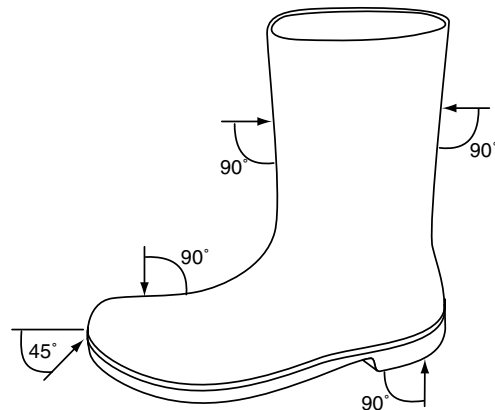
FIGURE 8.33.5.2 Test areas.
