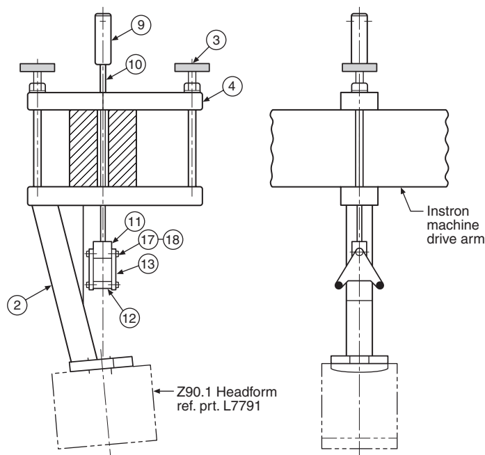
FIGURE 8.24.4.2 Retention system test setup.
