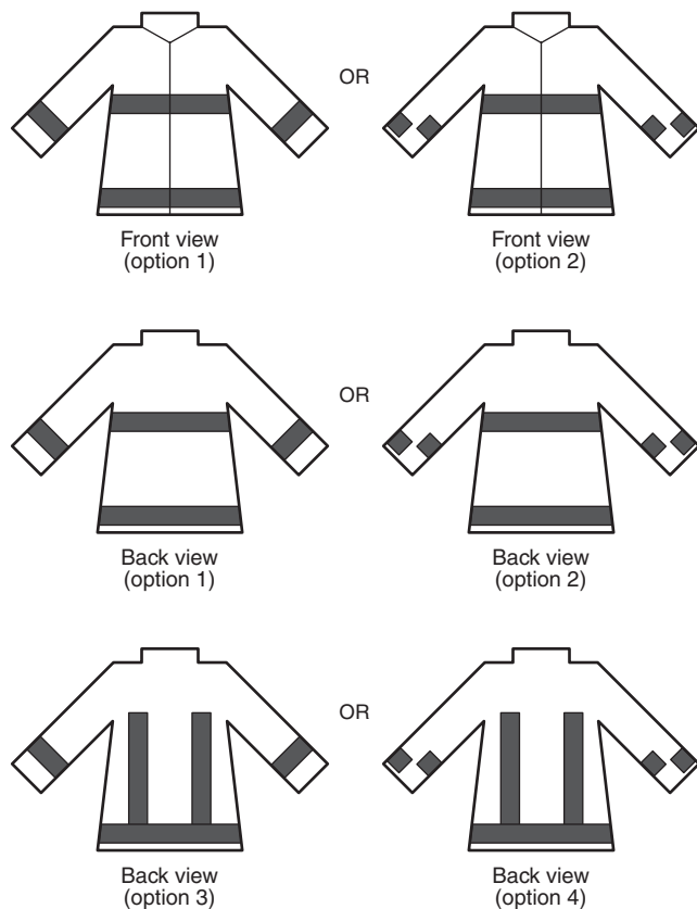
FIGURE 6.1.18.6 Minimum required coat trim patterns.
