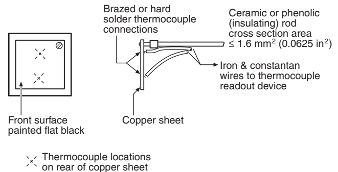
FIGURE 8.1.6.5 Radiant heat transducer.
