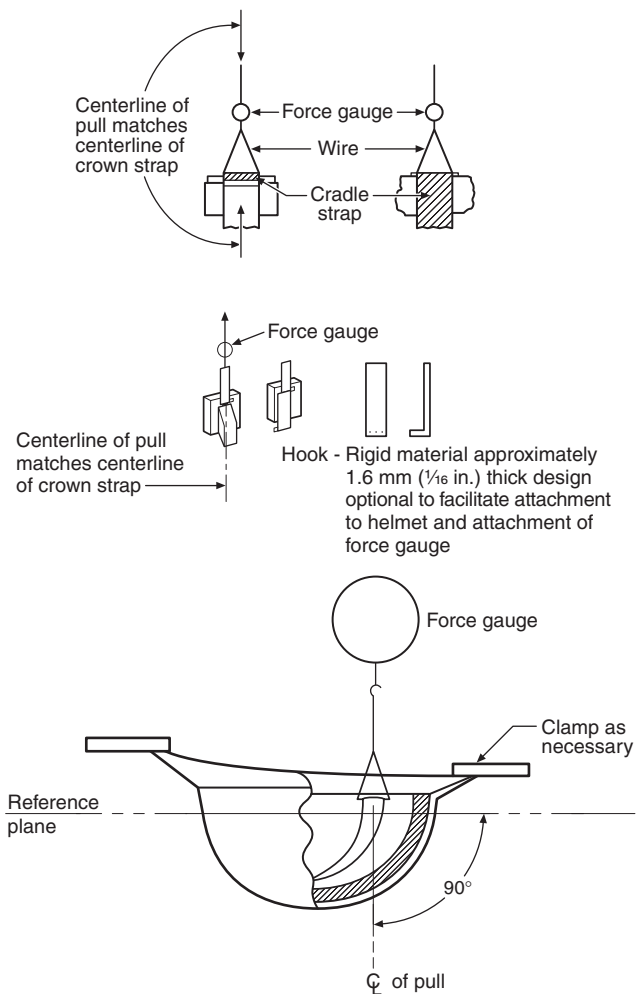
FIGURE 8.23.4 Suspension system test setup.
