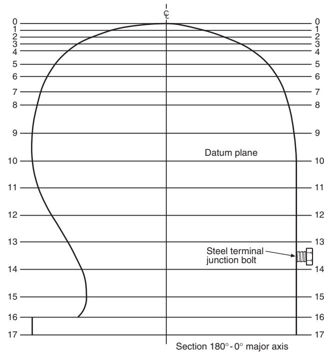
FIGURE 8.20.4.1(b) ISEA size 7 headform, side with modification for steel terminal junction bolt.
