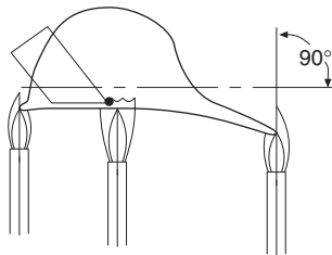
FIGURE 8.19.5.1.1 Test Procedure A.
