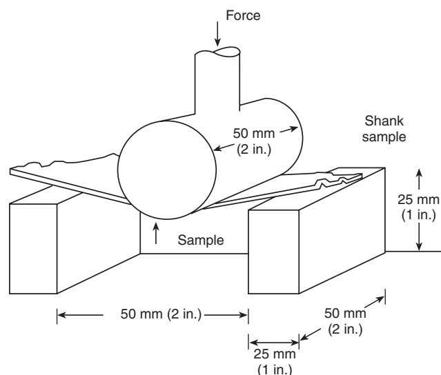
FIGURE 8.35.4 Shank bend test setup.
