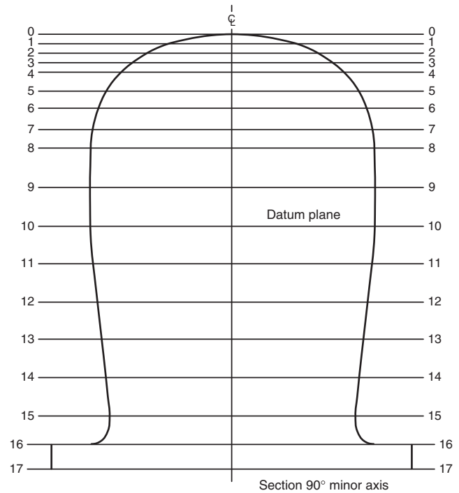
FIGURE 8.20.4.1(c) ISEA size 7 headform, front.
