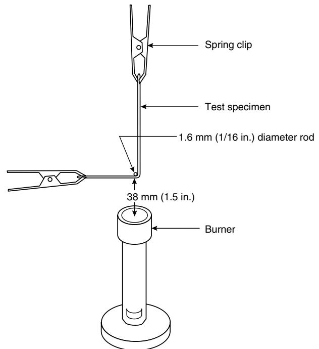
FIGURE 8.25.4.3 Relationship of test material to burner.
