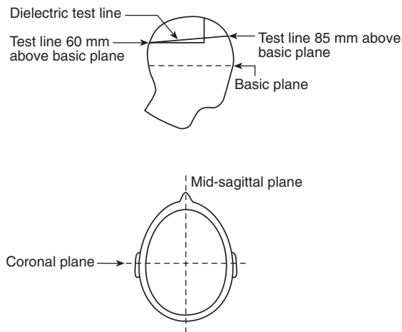
FIGURE 8.22.5.1.2 Test setup.
