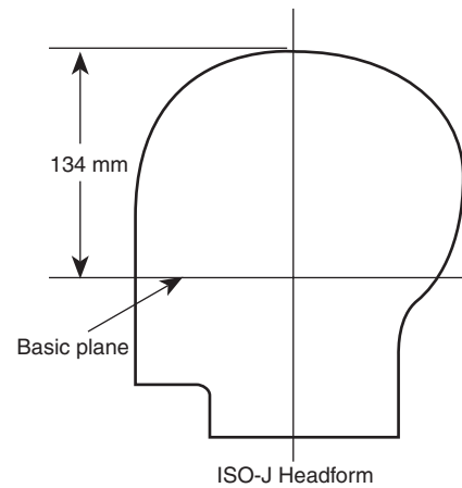
FIGURE 8.24.4.1 ISO size J headform.
