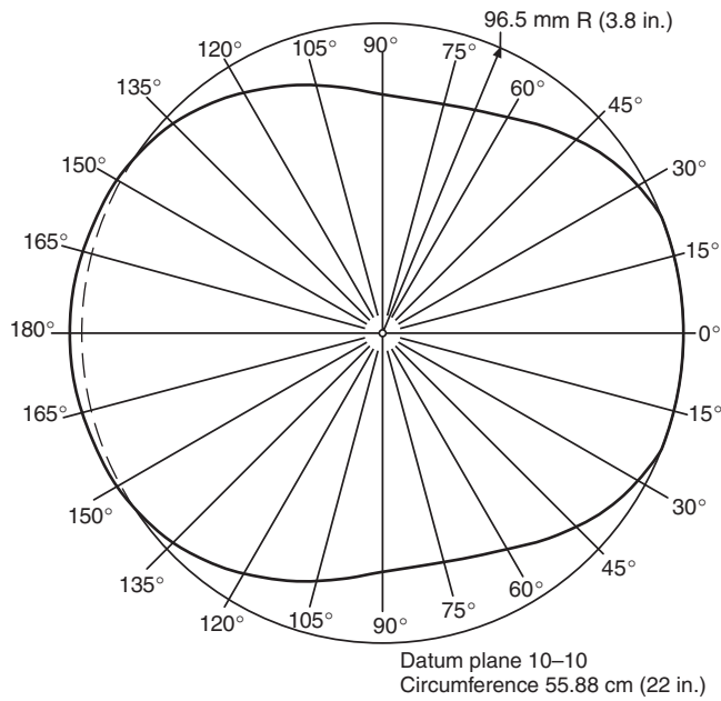
FIGURE 8.20.4.1(a) ISEA size 7 headform, top.
