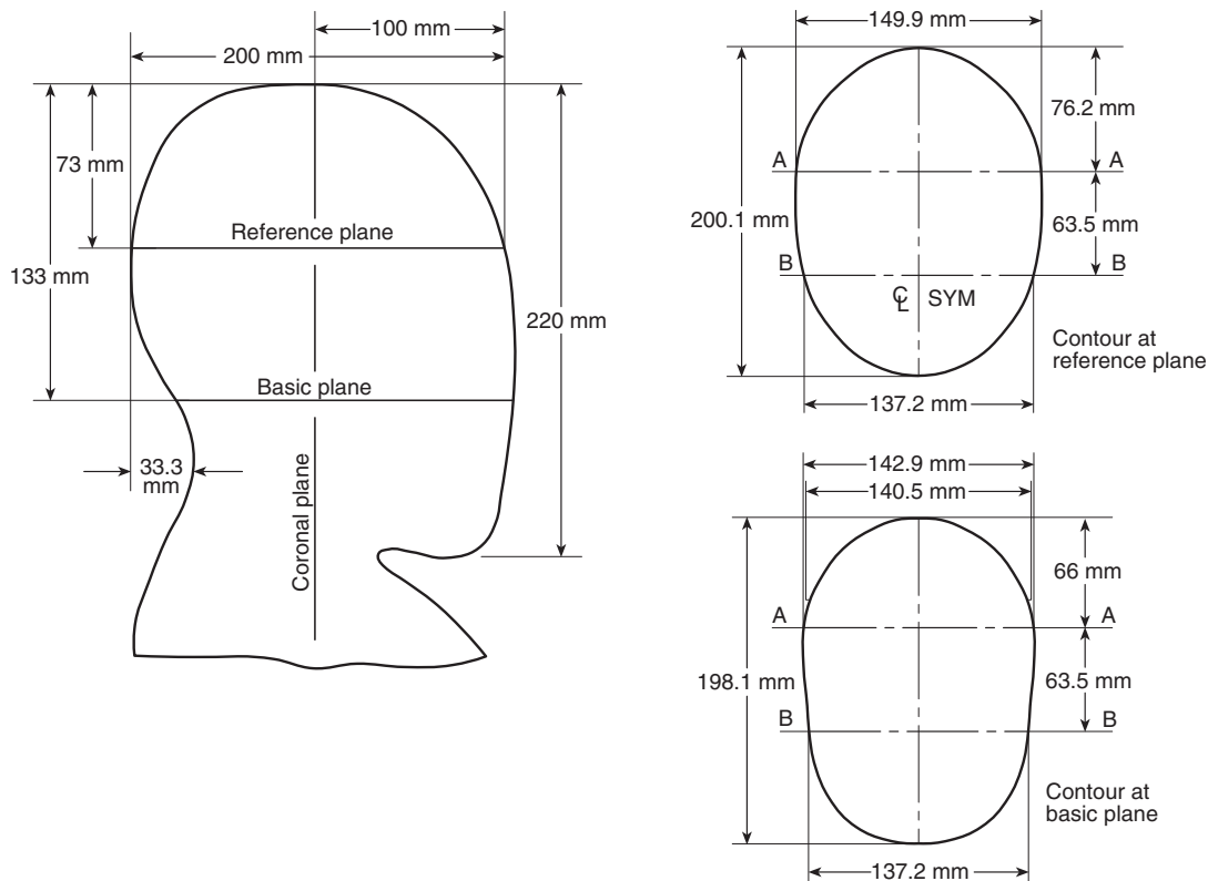
FIGURE 8.5.11.4 Thermal headform.
