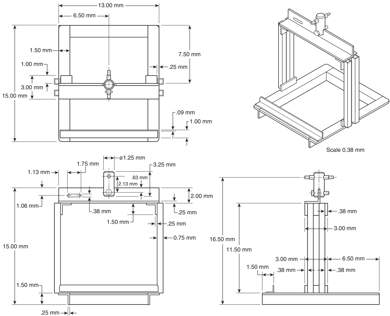
FIGURE A.8.43.4.1(a) Shell Retention Test Fixture.
