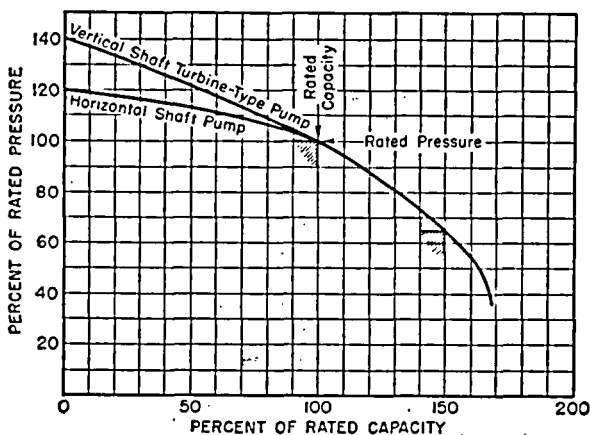
Fig. 13. Characteristic Curves.
