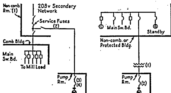
B—Electric Supply from Underground Utility Company Network.
