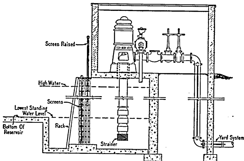
Fig. 201b. Vertical Shaft Turbine-Type Pump-Installation in Wet Pit.
