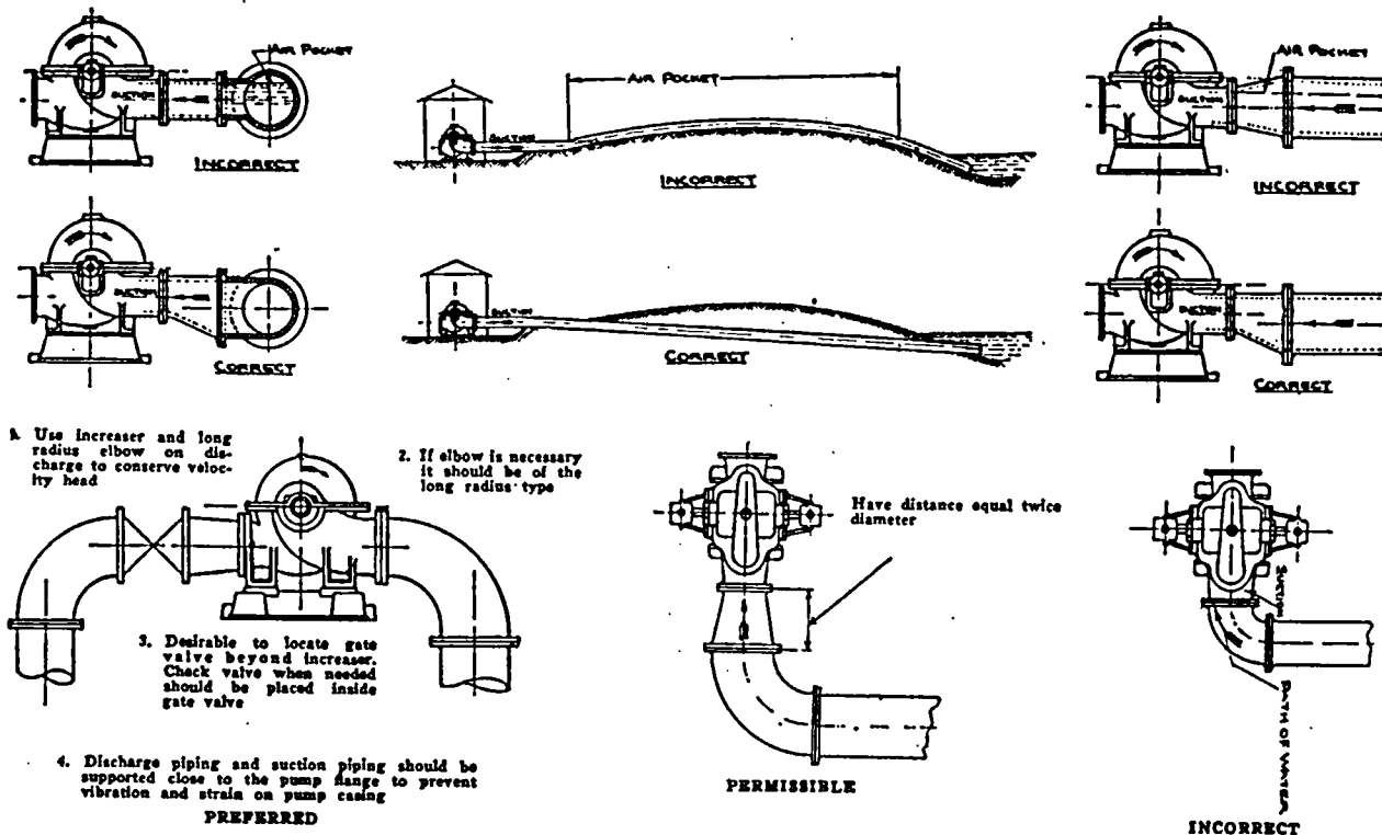
Fig. 114f. Correct and Incorrect Pump Suctions.
