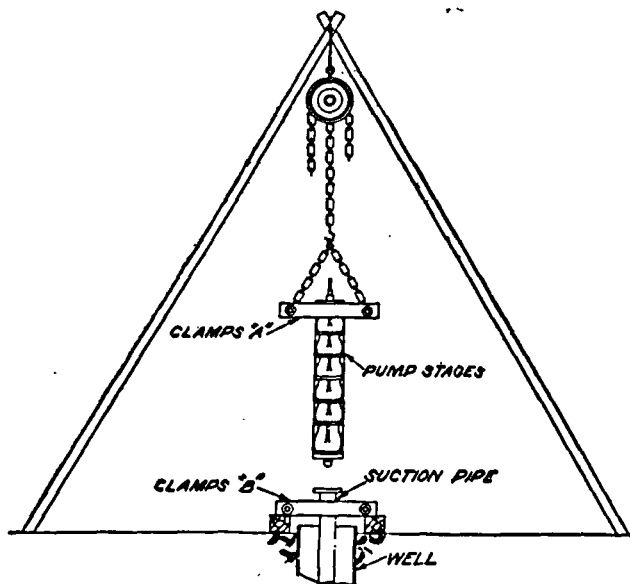
Fig. 234b-3. Installation of Pump Stages.
