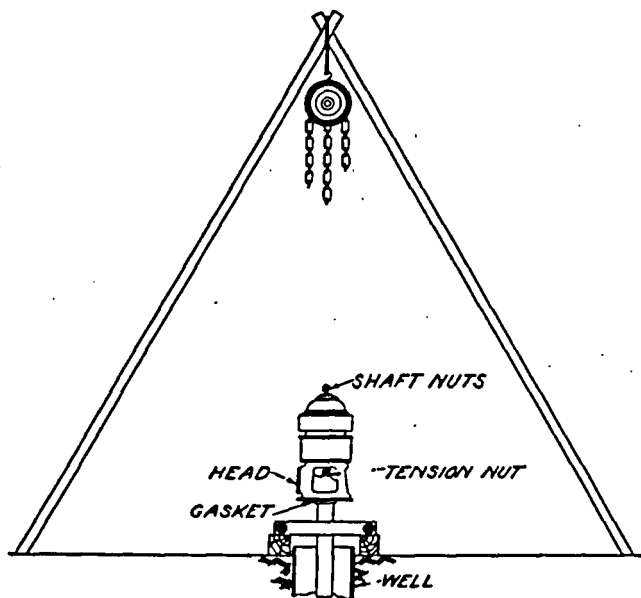
Fig. 234b-4. Installation Diagram—Top Section (Flange Type).
