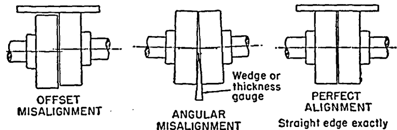
Fig. 112. Proper and Improper Shaft Alignment.
