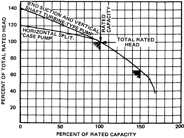
Figure A-3-2.1 Pump Characteristic Curves.
