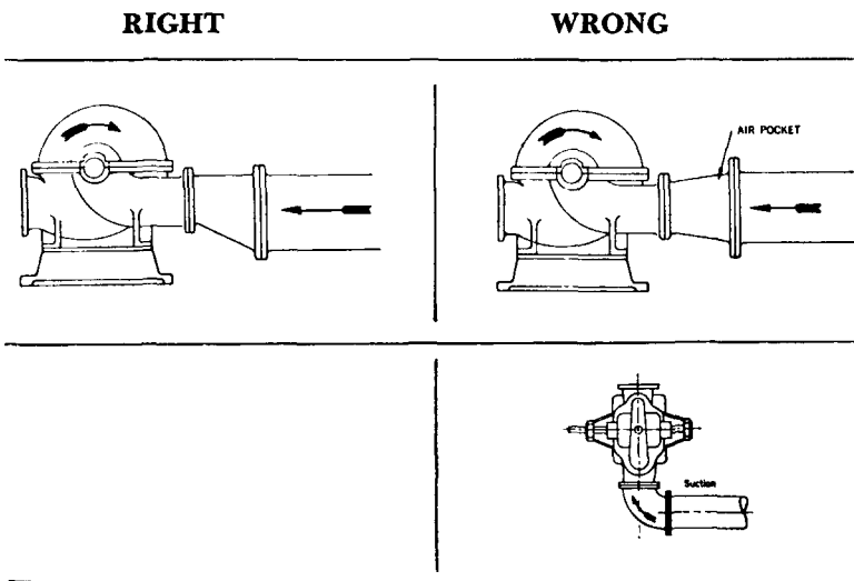
Figure A-2-9.6 Right and Wrong Pump Suctions.
