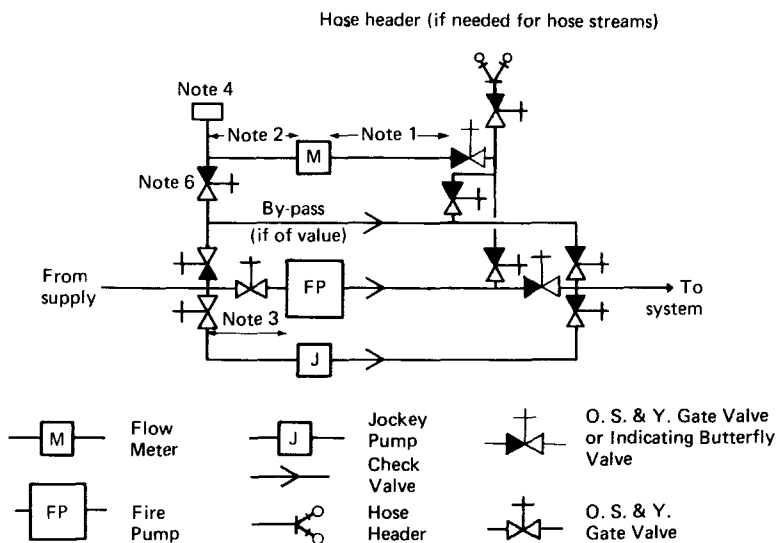
Figure A-2-13.2.1(b) Diagram of Arrangement for Measuring Fire Pump Water Flow with Meter, Discharge Water Return to Pump Suction. (Not Recommended, see Note 6.)
