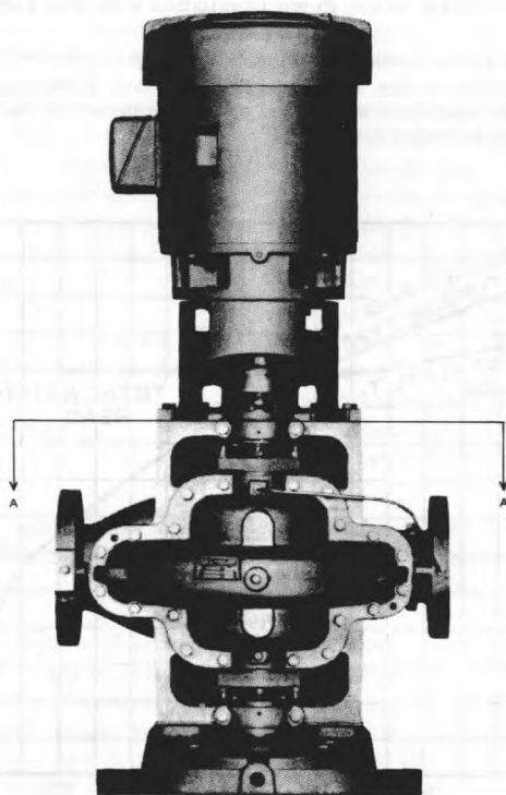
Figure A-2-16(c) Vertical Pump Shaft Rotation.
