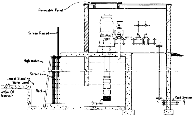
Figure A-4-2.2.2 Vertical Shaft Turbine-type Pump — Installation in a Wet Pit.
