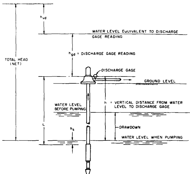
Figure A-1-8.5.8 Total Head of Vertical Turbine-type Fire Pumps.
