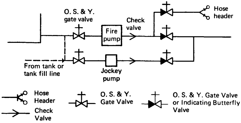
Figure A-2-19.3 Jockey Pump Installation with Fire Pump.
