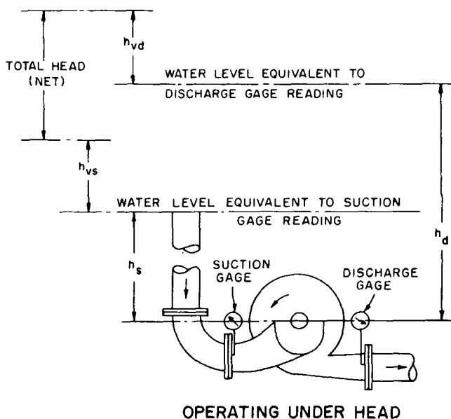
Figure A-1-8.5.7 Typical Head of Horizontal Shaft Centrifugal Fire Pumps.
