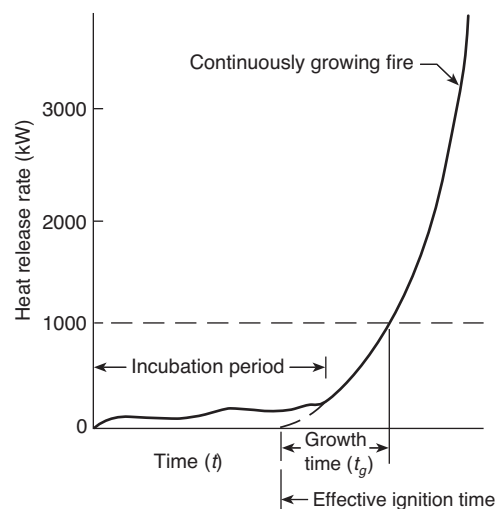
FIGURE 8.3.1 Conceptual Illustration of Continuous-Growth Fire.
