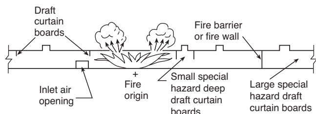
FIGURE A.1.1.1(a) Behavior of Combustion Products Under Vented and Curtained Roof.
