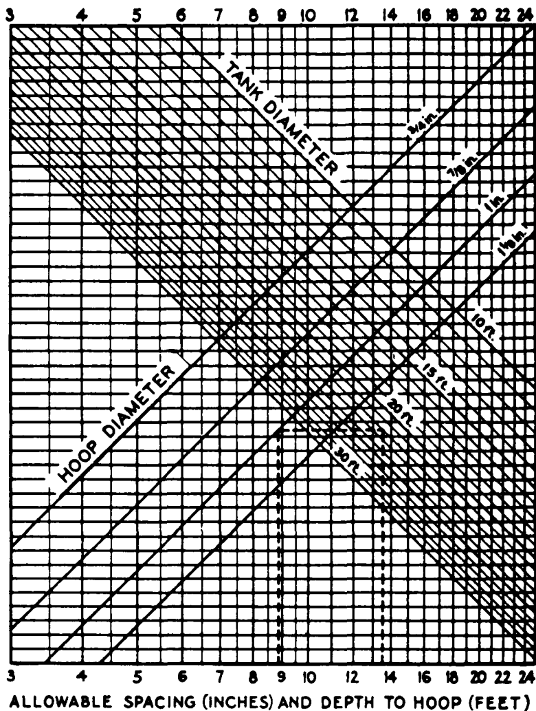
Figure 4-5.3. Hoop Spacing Diagram for Wood Tanks.
