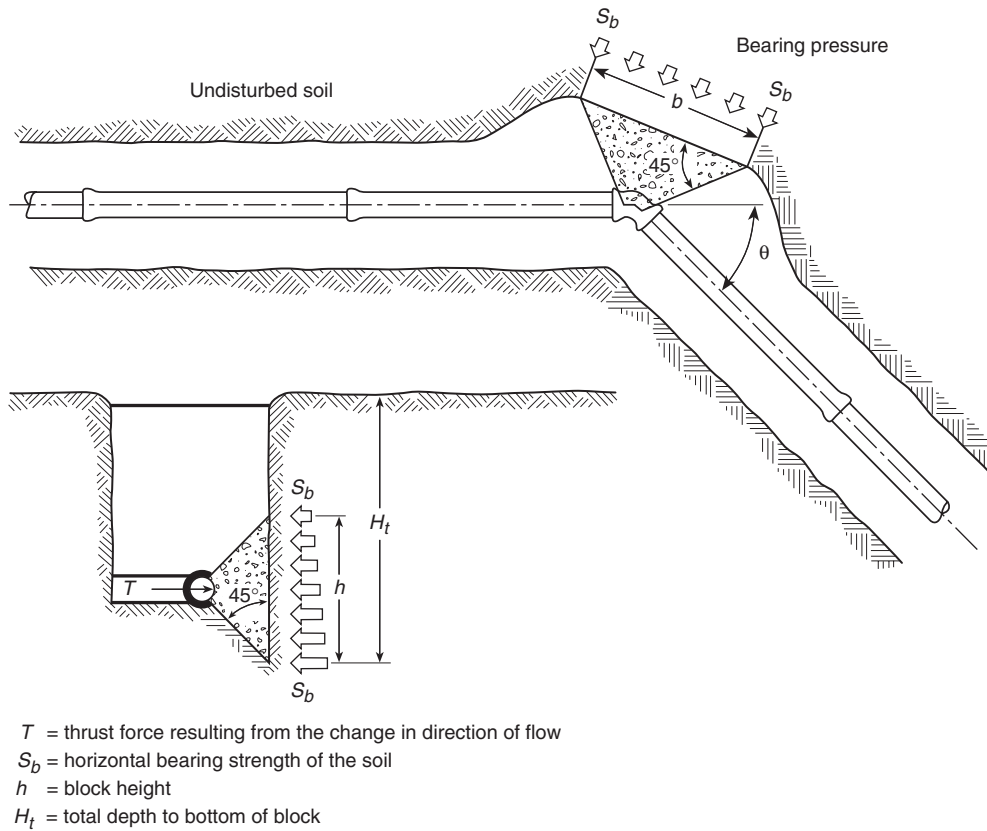
FIGURE A.10.8.2(b) Bearing Thrust Block.
