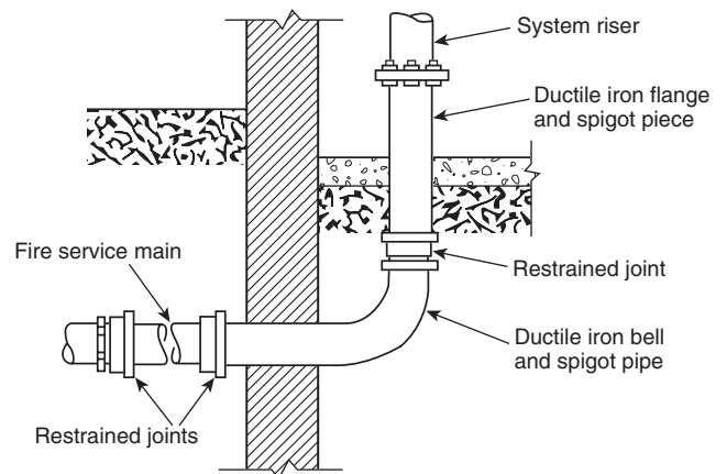
FIGURE A.10.8.3 Typical Connection to a Fire Protection System Riser Illustrating Restrained Joints.
