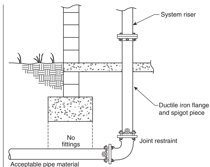
FIGURE A.10.6.5 Pipe Joint Location in Relation to Foundation Footings.
