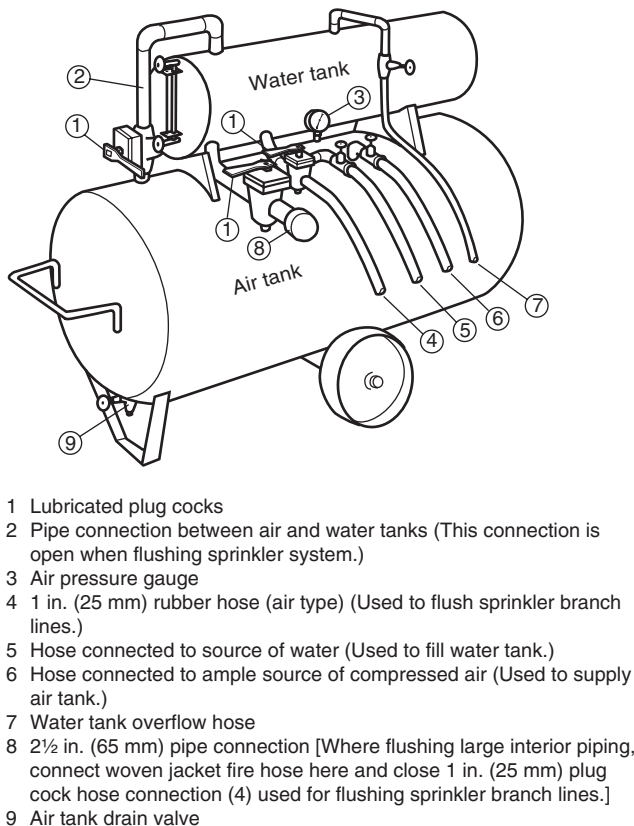
FIGURE D.5.4(a) Hydropneumatic Machine.
