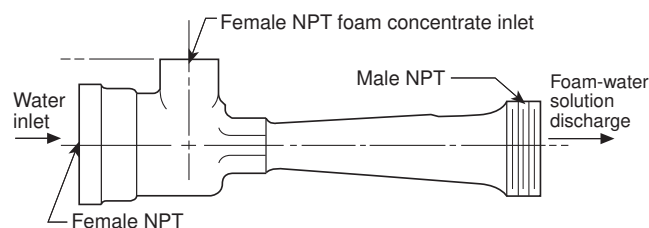
FIGURE A.3.3.35 Proportioner.
