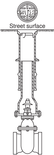
FIGURE A.13.1(i) Nonindicating-Type Gate Valve.
