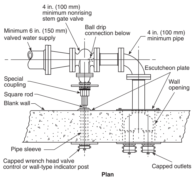
FIGURE A.3.3.13.4 Wall Hydrant.
