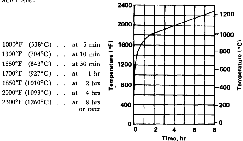
Figure 2-1.1 Time-Temperature Curve
