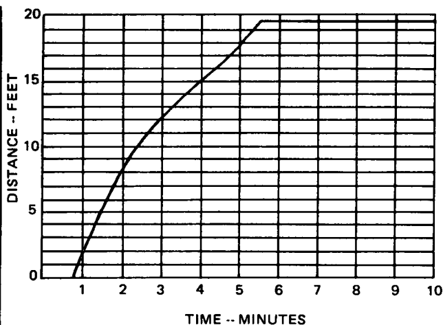
Figure 7 Time-Distance Curve for Flame Spread of Red Oak.
