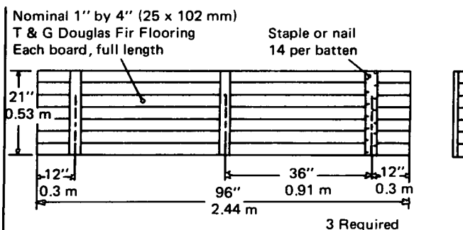
Figure A-5.2 Wood Deck for Coating Material.
