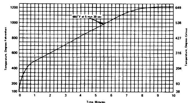
Figure 4 Time-Temperature Chart for Red Oak.
