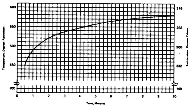
Figure 6 Time-Temperature Chart for Asbestos Cement Board.
