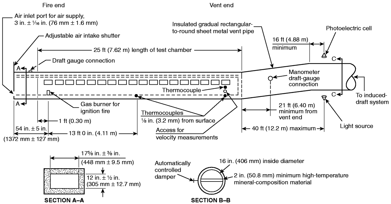
FIGURE 4.1.1(a) Fire Test Chamber.
