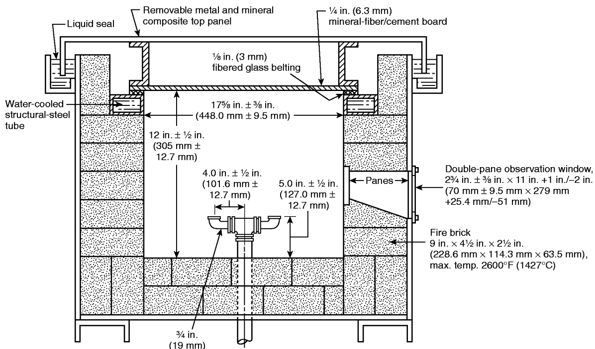
FIGURE 4.1.1(b) Side View of Fire Test Chamber.
