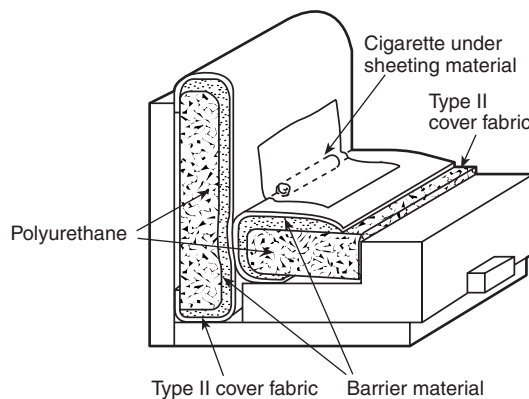
FIGURE 6.6.1.2 Barrier Materials Test Method.
