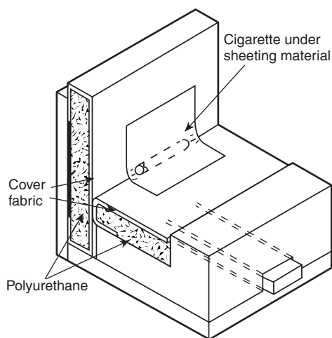
FIGURE 6.1.1 Cover Fabric Test Method.
