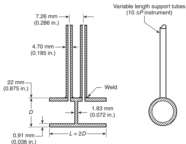
FIGURE 7.3.2.1 Bidirectional Probe.
