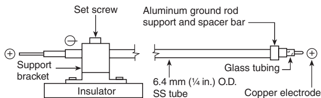
FIGURE 5.4.2.1(a) Plan View of the Spark Igniter.
