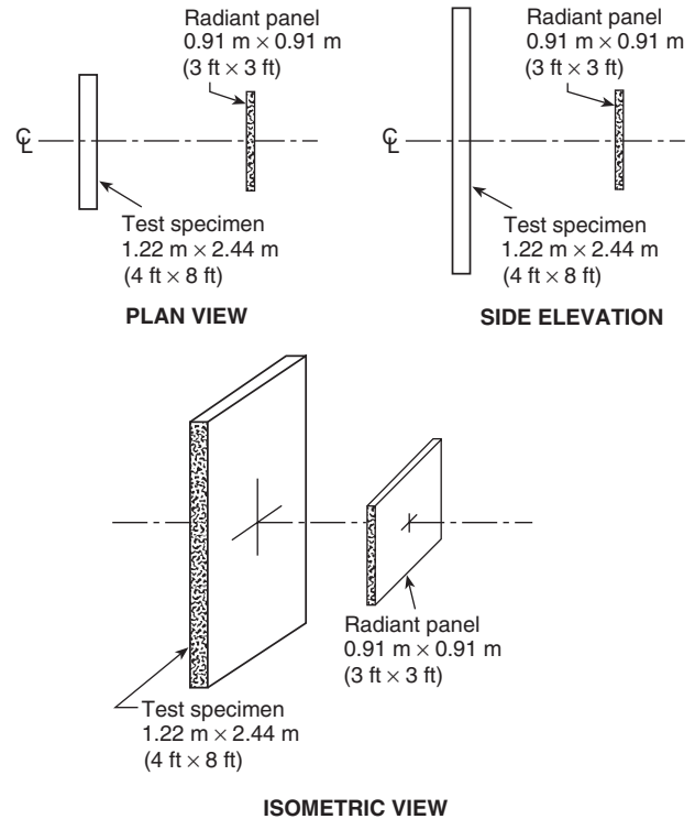
FIGURE 4.1 Spatial Relationship Between the Test Specimen and the Radiant Panel.
