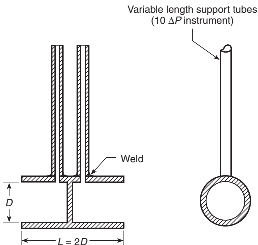
▲ FIGURE 7.3.2 Bidirectional Probe.
