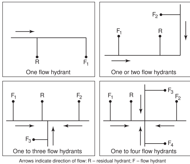
FIGURE 4.4.4 Suggested Test Layout for Hydrants.
