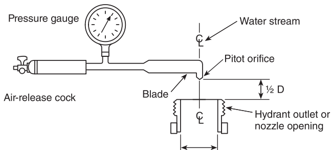
N FIGURE 4.8.3 Pitot Tube Position.
