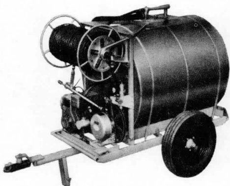
Trailer tanker, equipped with rotary, positive pump capable of pressures to 450 psi at delivery of 12 U.S. (10 Imp.) gpm. Tank holds 300 U.S. (250 Imp.) gallons and is fitted with live hose reel and filling ejector.
