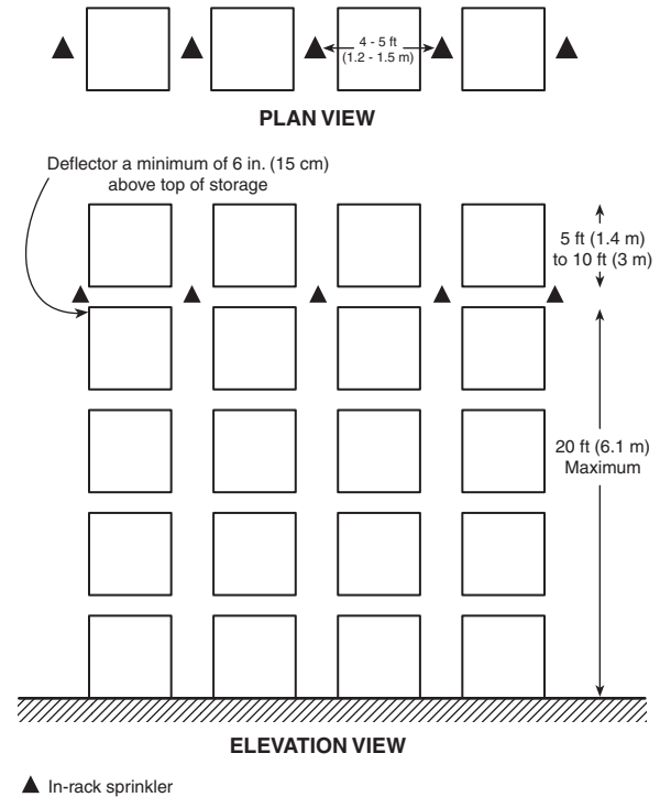
N FIGURE 16.6.6.1(a) Single-Row Rack Sprinkler Layout for Design Scheme “F.”
