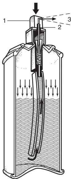
FIGURE A.3.3.2 An aerosol can (cutaway view). When the plunger (1) is pressed, a hole in the valve (2) allows a pressurized mixture of product and propellant (3) to flow through the plunger's exit orifice. (Source: Fire Protection Handbook , 18th edition)
