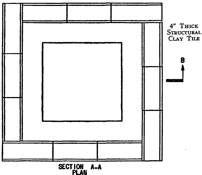
Installation of Downflow Furnace on Combustible Floor Figure 3.
