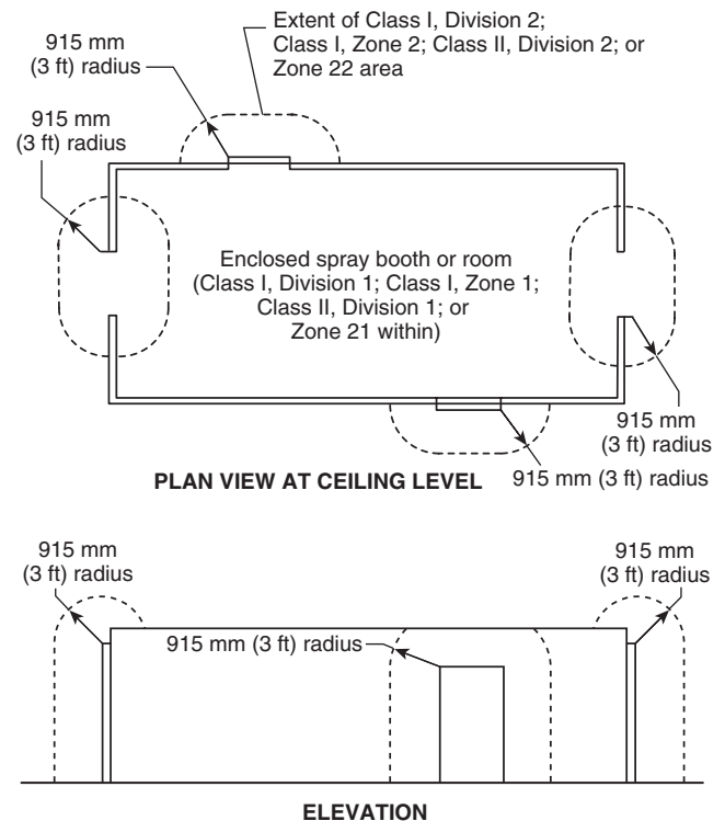
FIGURE 6.5.4 Class I, Division 2; Class I, Zone 2; Class II, Division 2; or Zone 22 Locations Adjacent to an Enclosed Spray Booth or Spray Room.
