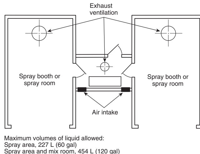
FIGURE 8.3.4(b) Mixing Room Within 1830 mm (6 ft) of Spray Area and with Direct Entry to Spray Area, Including Maximum Volume of Liquid Allowed.
