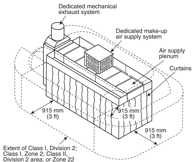
FIGURE 14.3.5.1 Class I, Division 2; Class I, Zone 2; Class II, Division 2; or Zone 22 Locations Adjacent to a Limited Finishing Workstation.
