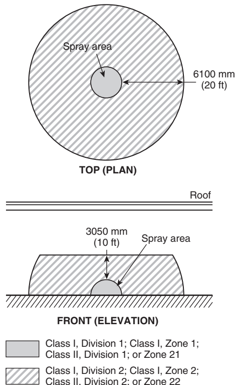
FIGURE 6.5.1 Electrical Area Classification for Unenclosed Spray Areas.
