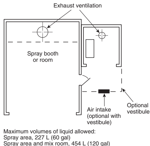
FIGURE 8.3.4(a) Mixing Room Within 1830 mm (6 ft) of Spray Area, Including Maximum Volume of Liquid Allowed.
