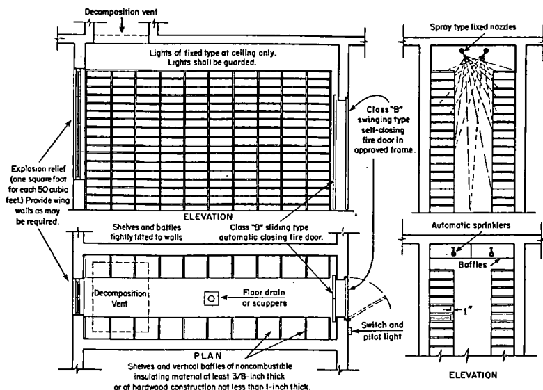
Fig. 4. Archival Vault.
