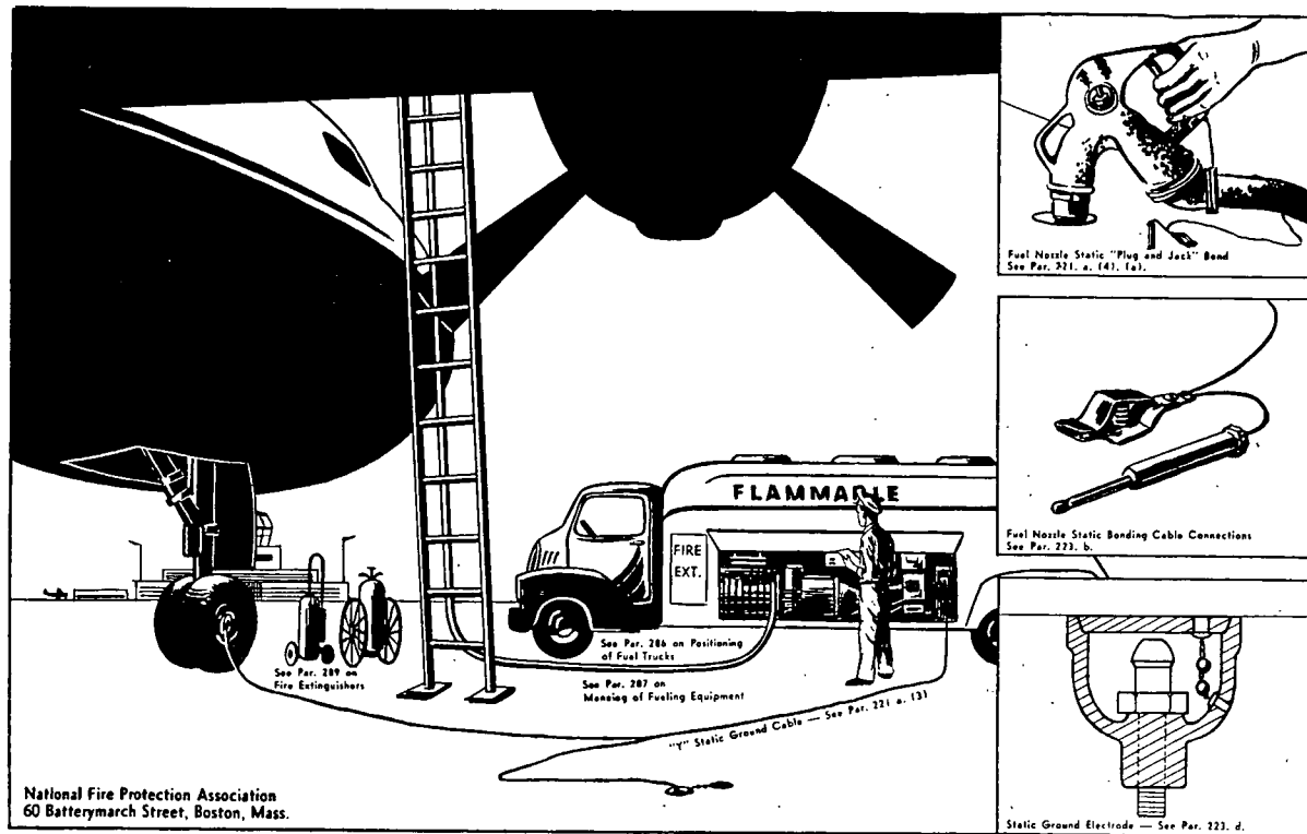
Figure 1. A typical over-the-wing fuel servicing operation from an aircraft fuel servicing tank vehicle show-
