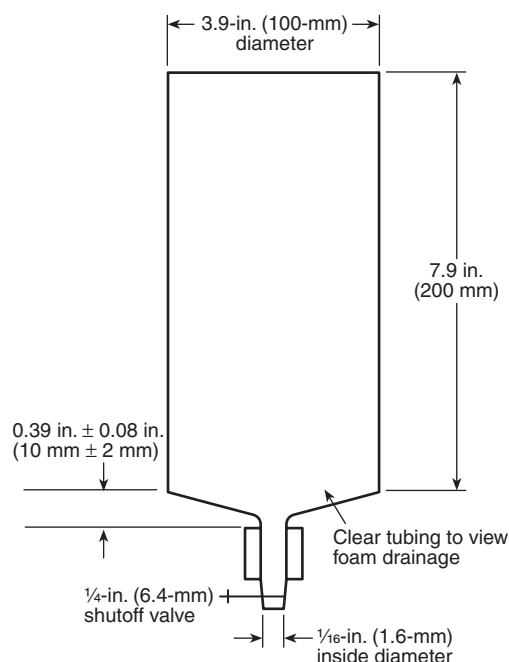
FIGURE 6.3.3.1.2 1600 mL Foam Sample Container.
