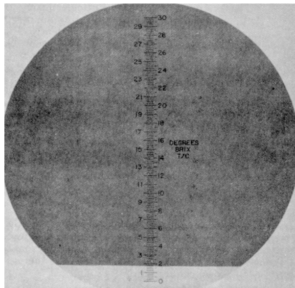
FIGURE A.6.2.2(c) Illustrating the Field of View by Looking Into the Refractometer Shown in Figures A.6.2.2(a) and A.6.2.2(b) Containing a 6 Percent AFFF Solution. The Dark Intersects the Scale at 1.7, and this Value Is Recorded as the Reading for a 6 Percent Concentration.
