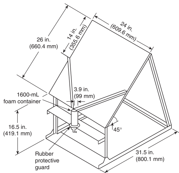
FIGURE 6.3.3.1.1 Foam Sample Collector.
