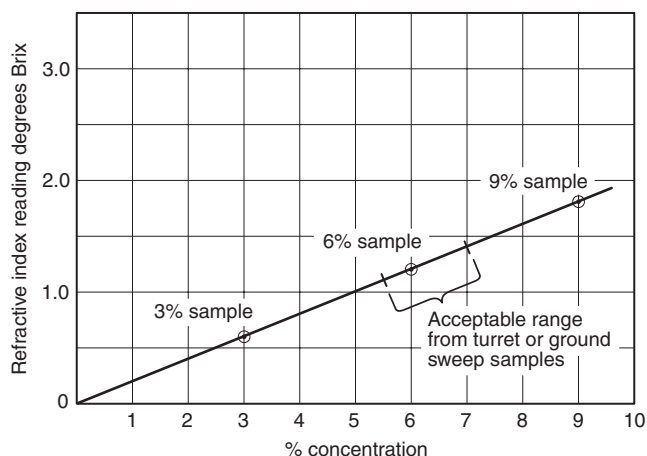
FIGURE A.6.3.2(a) Typical Graph Using AFFP (6%).
