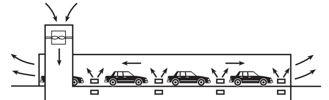
FIGURE I.3.1(b) Semitransverse Supply Ventilation System.
