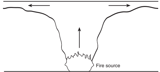
FIGURE A.3.3.5(a) Tunnel Fire Under Natural Ventilation and Zero Percent Grade.
