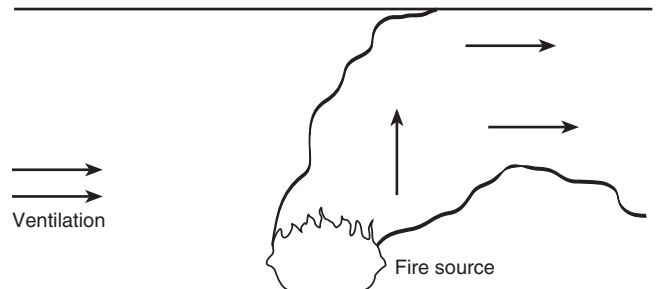
FIGURE A.3.3.5(c) Tunnel Fire Sufficiently Ventilated to Prevent Backlayering.
