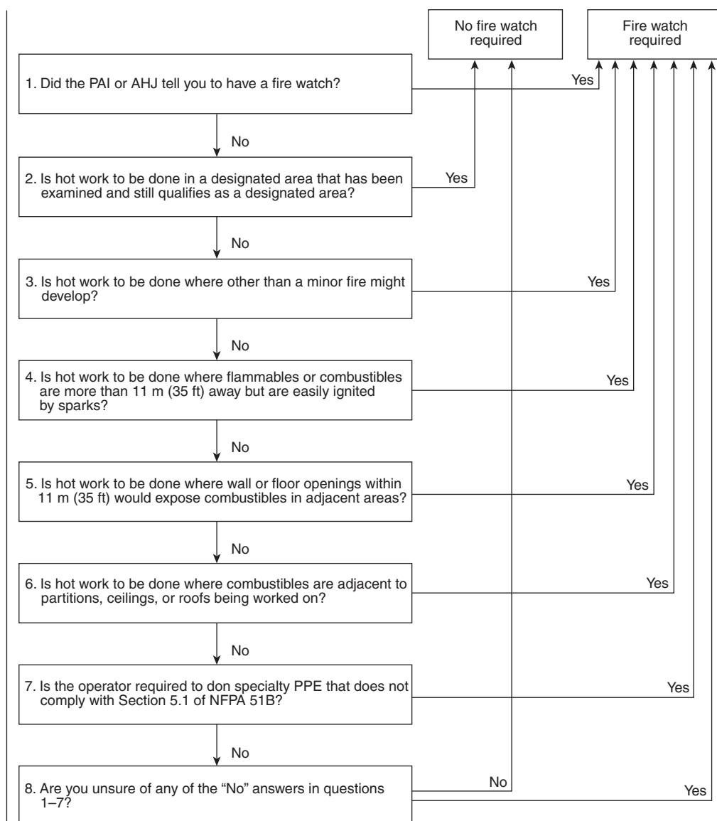
FIGURE A.5.5.1 Fire Watch Decision Tree.
