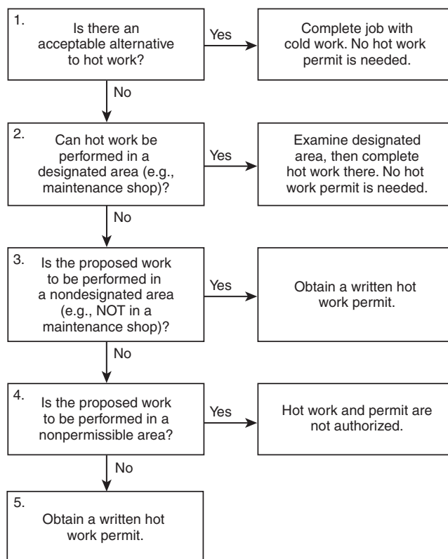
FIGURE A.5.4 Hot Work Permit Decision Tree.
