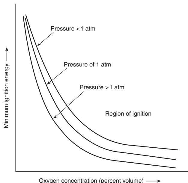
FIGURE E.3.2.2 Minimum Ignition Energy Behavior of Combustibles in Oxygen-Diluent Atmospheres at Different Pressures.
