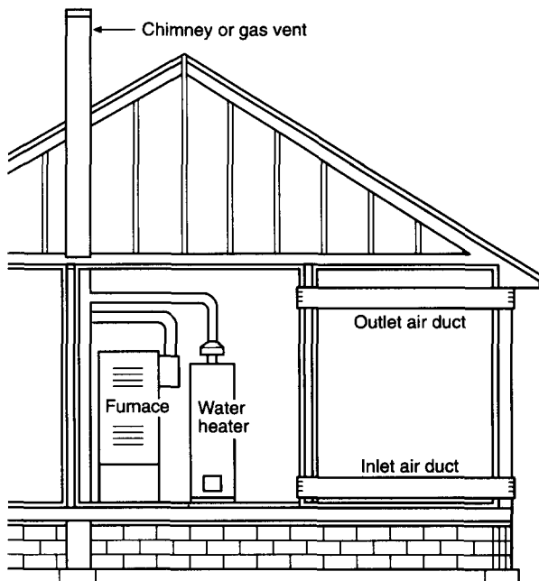
Figure 4. Equipment Located in Confined Spaces; All Air from Outdoors. See 5.3.3(b).
