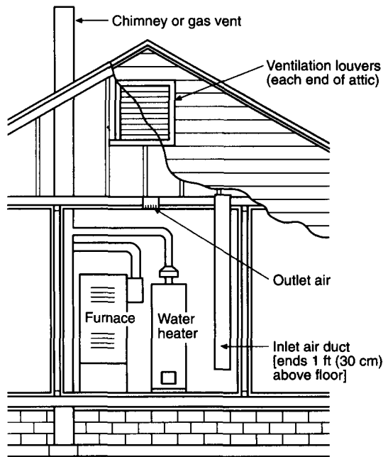
Figure 3. Equipment Located in Confined Spaces; All Air from Outdoors Through Ventilated Attic. See 5.3.3(b).
