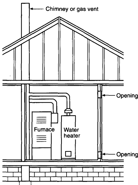
Figure 1. Equipment Located in Confined Spaces; All Air from Inside the Building. See 5.3.3(a).
