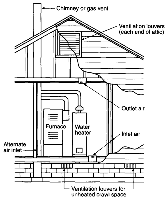
Figure 2. Equipment Located in Confined Spaces; All Air from Outdoors — Inlet Air from Ventilated Crawl Space and Outlet Air to Ventilated Attic. See 5.3.3(b).
