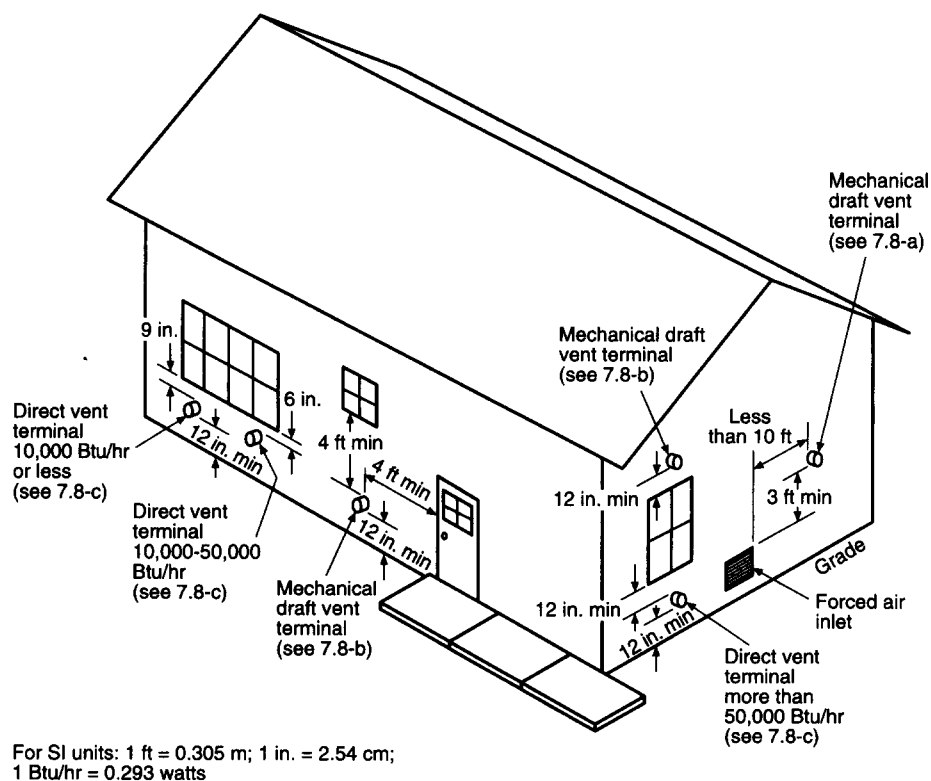
Figure A.7.8. Exit Terminals of Mechanical Draft and Direct-Vent Venting Systems.
