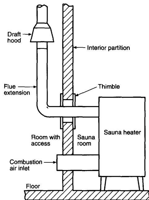
Figure 9. Typical Sauna Heater Installation.
