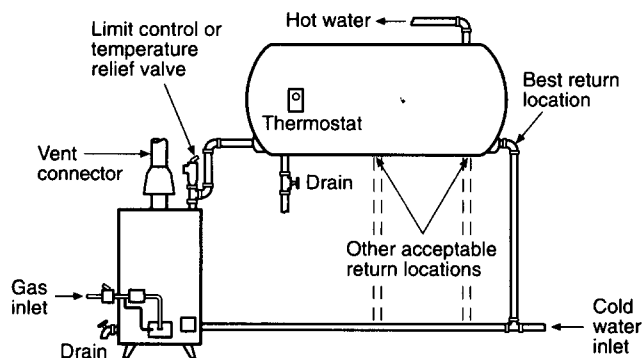
Figure 11. Typical Gravity Circulating Tank-Type Installation.
