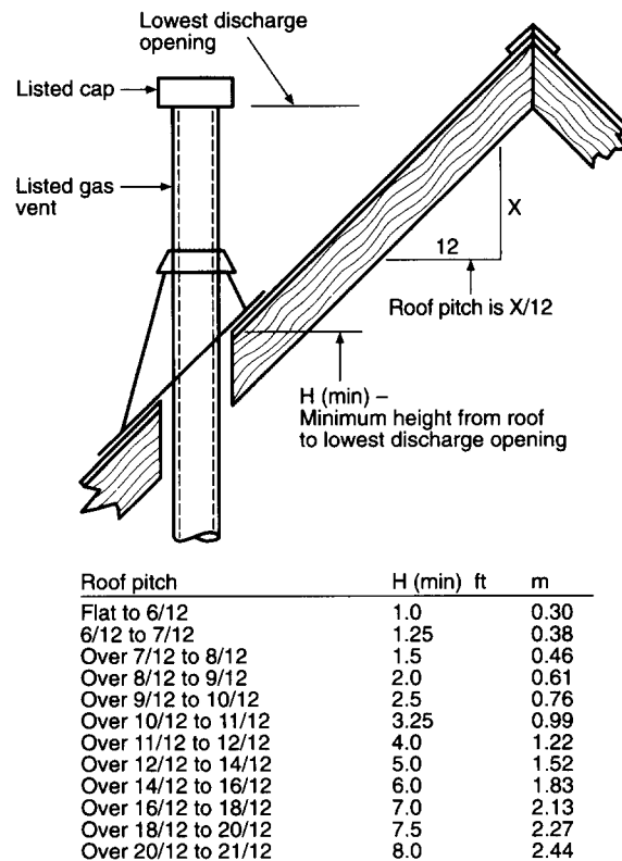
Figure 13. Gas Vent Termination Locations for Listed Caps 12 in. (300 mm) or Less in Size at Least 8 ft (2.4 m) from a Vertical Wall.
