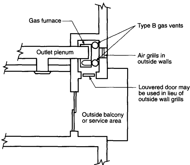
Figure 14. Plan View of Practical Separation Method for Multistory Gas Venting.
