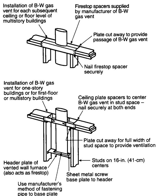
Figure 10. Installation of Type B-W Gas Vents for Vented Wall Furnaces.
