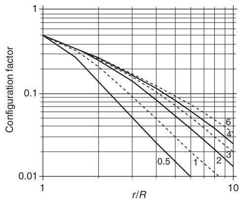
FIGURE 10.3.4.1(a) Configuration Factor for a Vertical Target and a Vertical Cylindrical Radiator.
