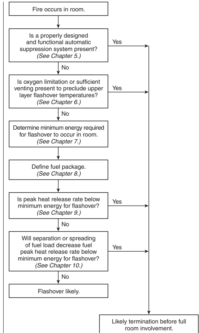
FIGURE 4.2 Flowchart for Use of NFPA 555.
