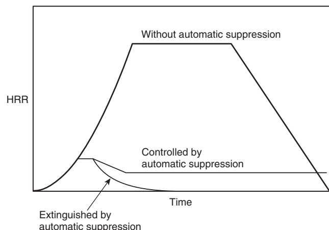
FIGURE 5.2 Effect of Automatic Fire Suppression Systems on Heat Release Rate. (Source: SFPE Engineering Guide to Performance-Based Fire Protection Analysis and Design of Buildings , Figure 9-3.)
