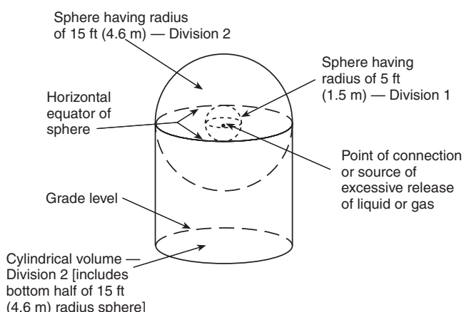
FIGURE A.4.5.2.2 Extent of Electrically Classified Area. (See Table 4.5.2.2.) [58:Figure A.6.23.2.3]
