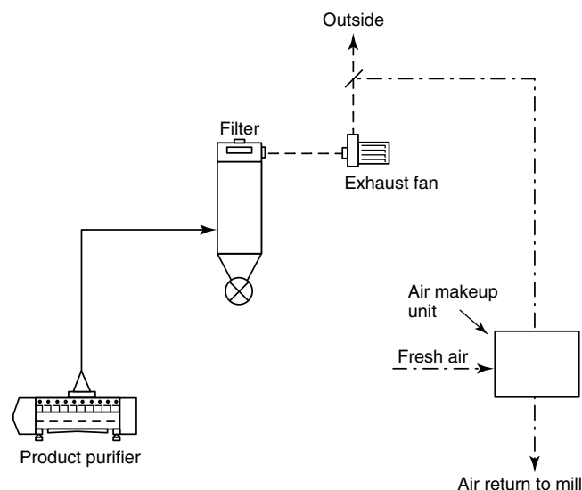
FIGURE A.8.3.4.1.3.5 Flow Diagram of Typical Product Purifier.
