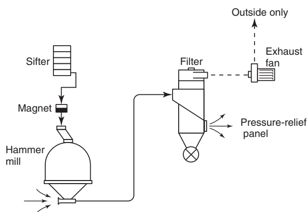
FIGURE A.8.3.4.1.3.4 Flow Diagram of Typical Hammer Mill Filter.
