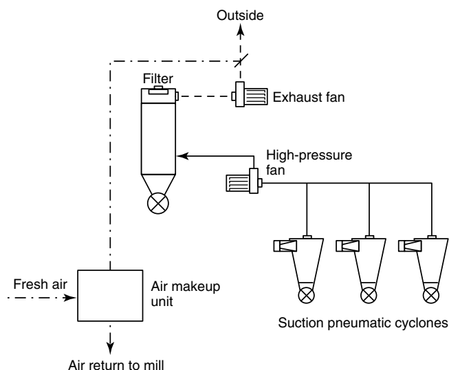
FIGURE A.8.3.4.1.3.3 Flow Diagram of Typical Pneumatic Filter Cyclone.
